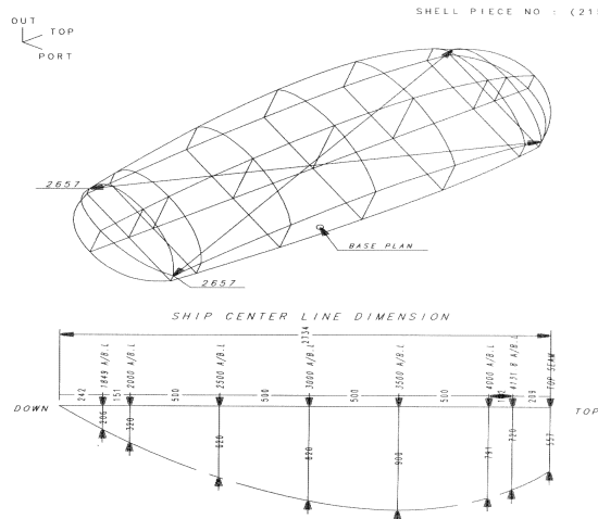
Figure 5 Bending templates for a shell plate
