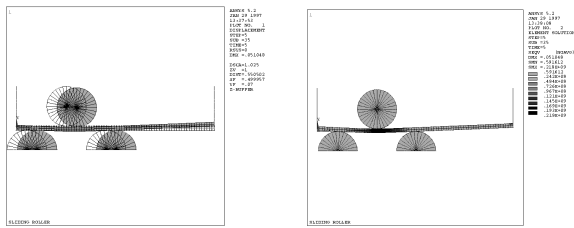
(a) Deformed shape (b) Equivalent strain distribution Figure 10 Configuration of roller bending procedure.
