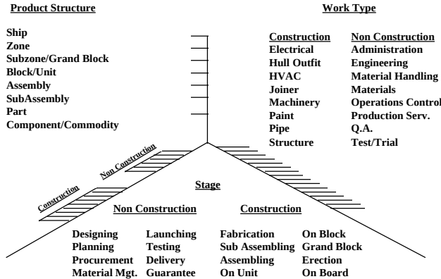
Figure 2. GPWBS system.
