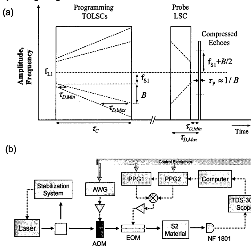
Figure 11. (a) The programming approach using LSCs. (b) The experimental setup for the demonstrations.
