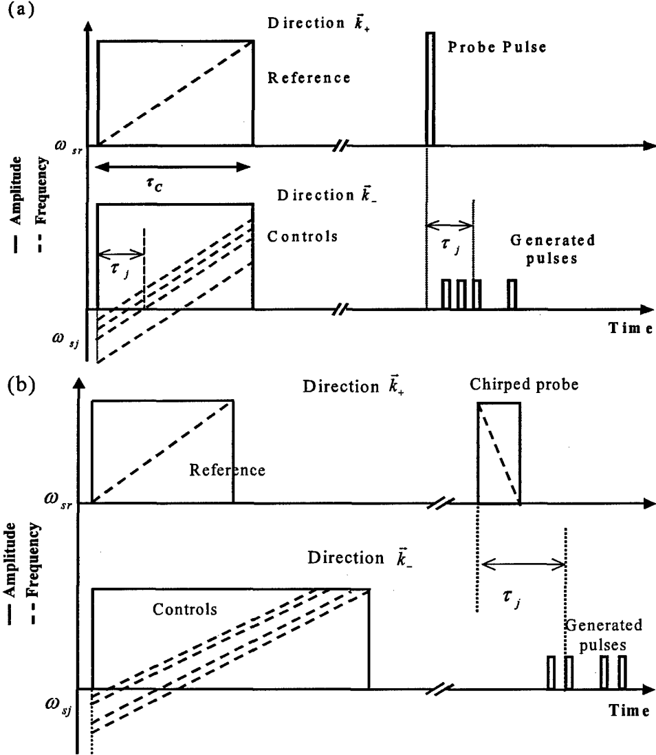
Figure 1. The TOLFC pulse shaping and AWG processes. Multiple frequency-chirped controls with different frequency offset in direction -k are temporally overlapped with chirped reference in direction k . After dephasing, a brief or chirped probe in direction k is diffracted by the spatial spectral grating producing multiple echoes in direction -k with delays corresponding to the frequency offset of controls. (a) The probe is a brief pulse, and (b) the probe is a downward frequency chirped pulse.
