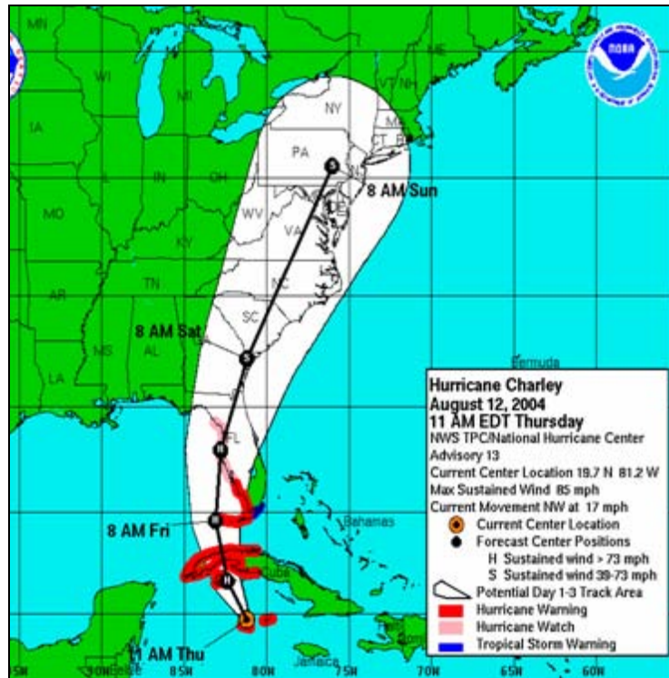
Figure 7. Five-day Hurricane Charlie Watch/Warning valid at 15 UTC 12 Aug 2004 (from Knaff and DeMaria 2005).
