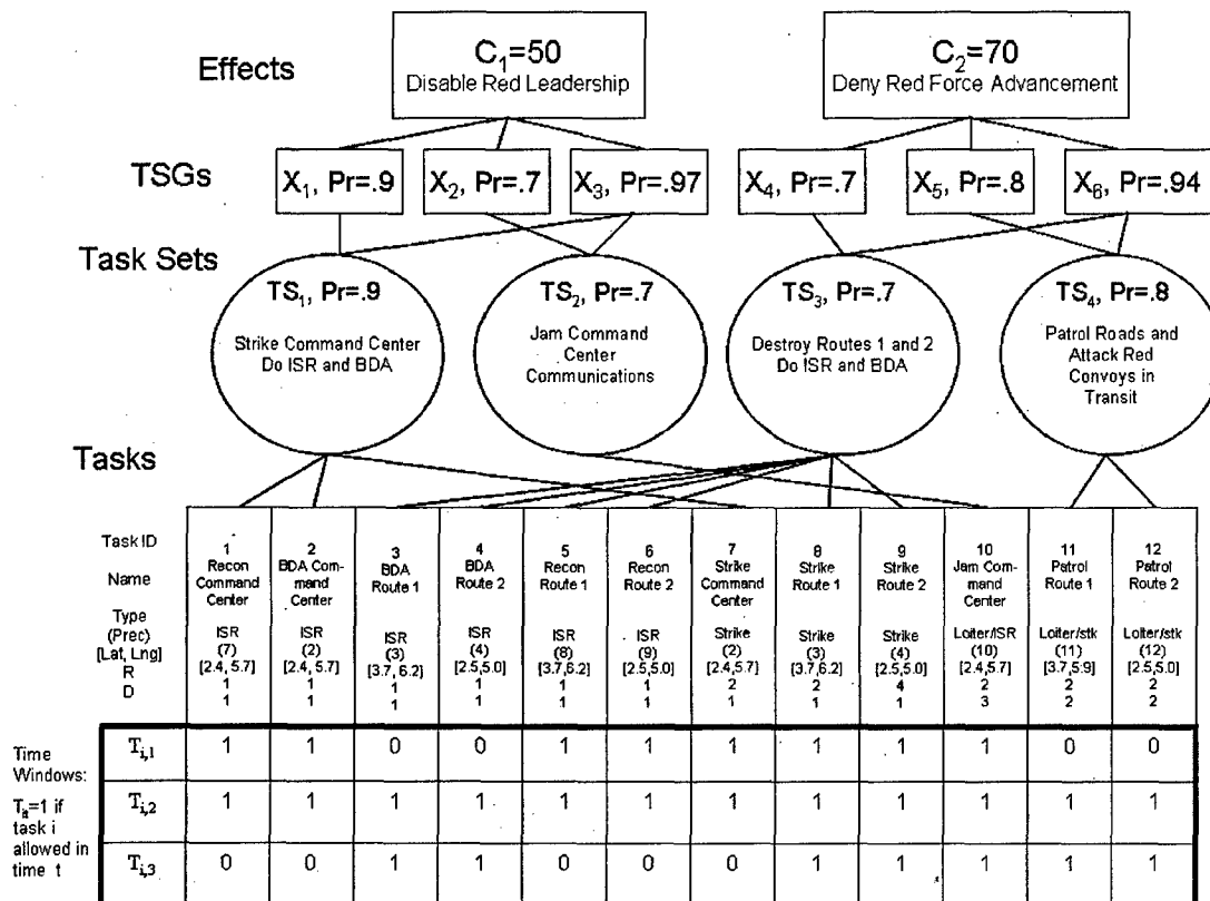
Figure 3-3: Small EBO Model Example
