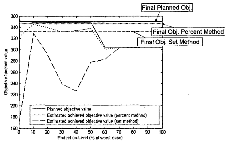
(b) Expected Achieved Value
