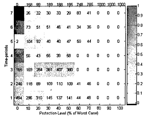
(b) Bertsimas/Sim Hazard Rate Plot
