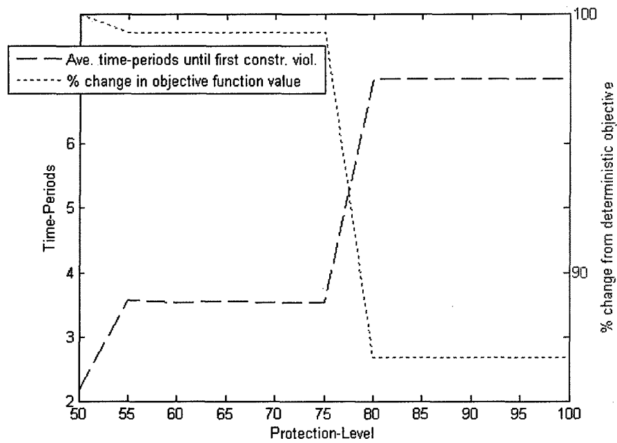
(a) Chance-Constrained Objective Function and Time until Failure
