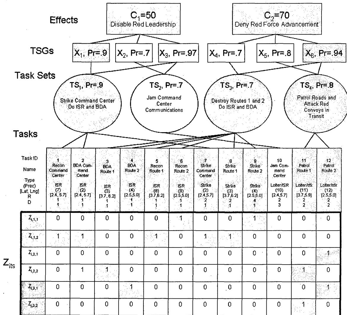
Figure 3-5: Small EBO Model Example Results
