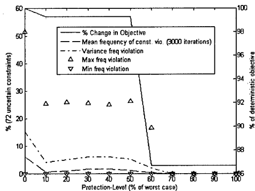
(c) Planned Objective Value and Freq. Constr. Viol.
