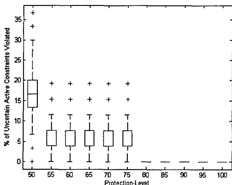
(c) Chance-Constrained Number of Active Constraints Violated
