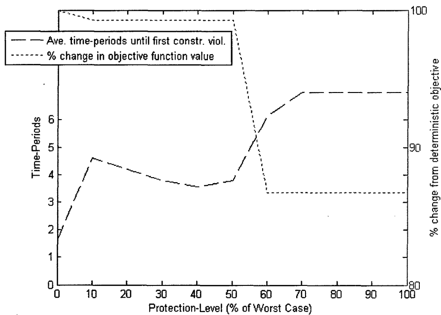
(b) Bertsimas/Sim Objective Function and Time until Failure
