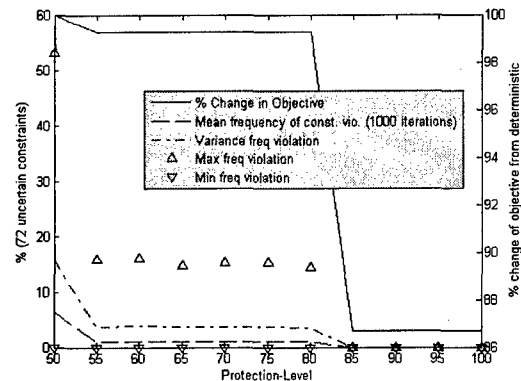
(b) Normal Obj. Function and Freq. Viol
