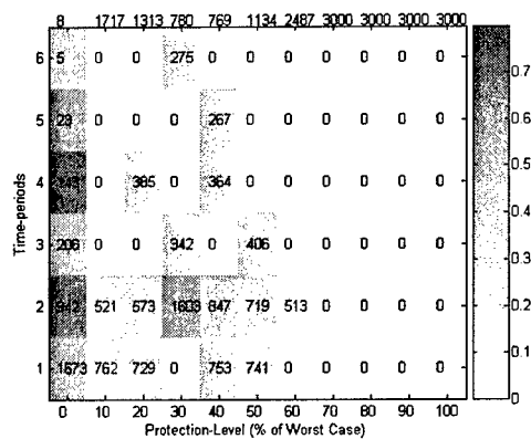
(a) Hazard Rate Plot
