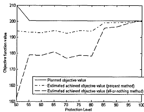
(c) Chance-Constrained Achieved Obj. Func.
