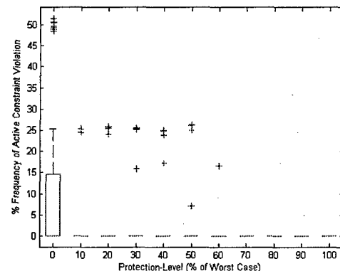
(b) Bertsimas/Sim Frequency of Active Constraint Violation
