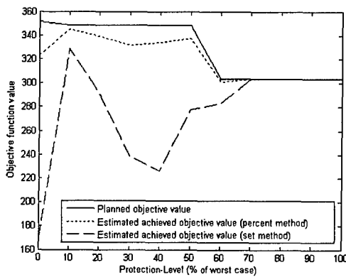
(e) Uniform Estimated Achieved Obj. Func.
