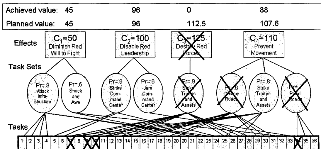
Figure 4-13: Set Method Performance
