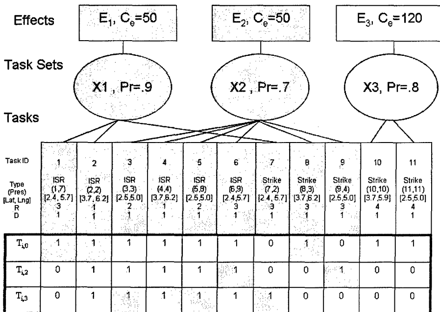
(b) Plan at Protection-Level 10
