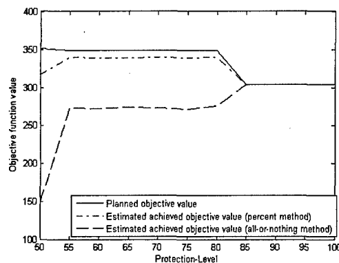
(f) Normal Estimated Achieved Obj. Func.
