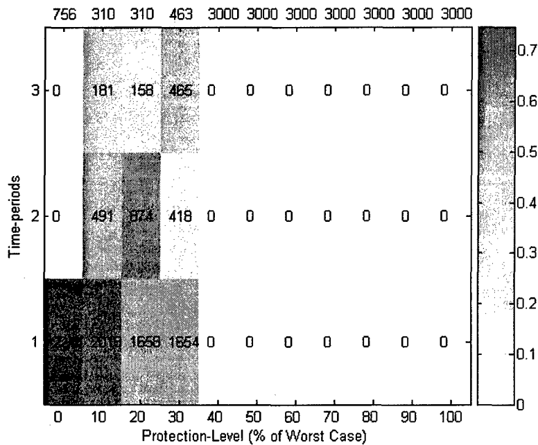
(b) Hazard Rate Plot
