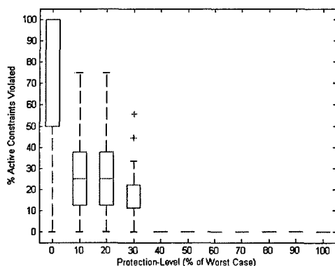
(c) Percent of ACTIVE Constraints
