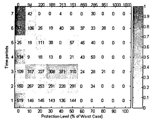
(b) Bertsimas/Sim Hazard Rate Plot
