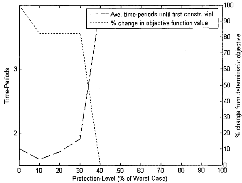
(a) Time Until Failure and Obj Value
