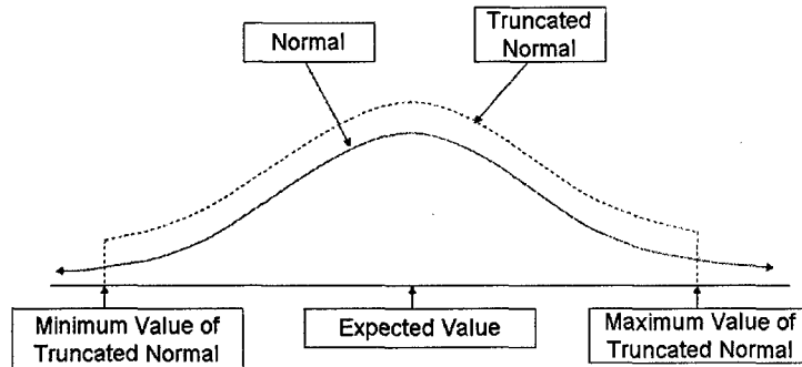
Figure 4-21: Normal vs. Truncated Normal Distribution
