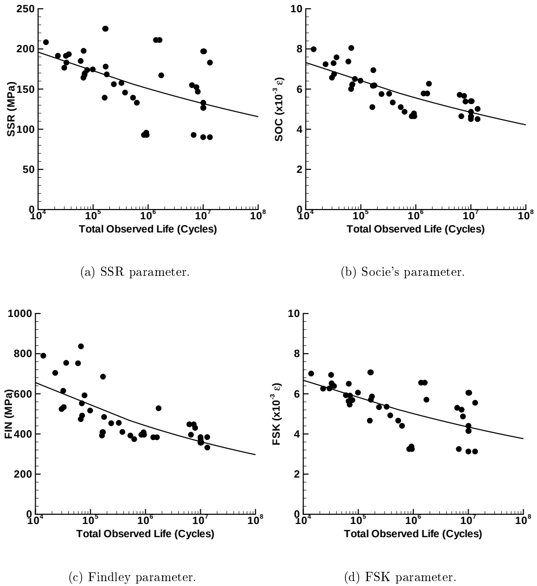
Figure 6.1. Comparison of uniaxial data and fretting data with different lifing parameters.
