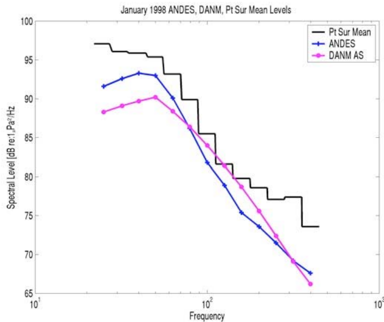
Figure 18. Mean levels: DANM AS, ANDES, and Point Sur in situ passband for January 1998
