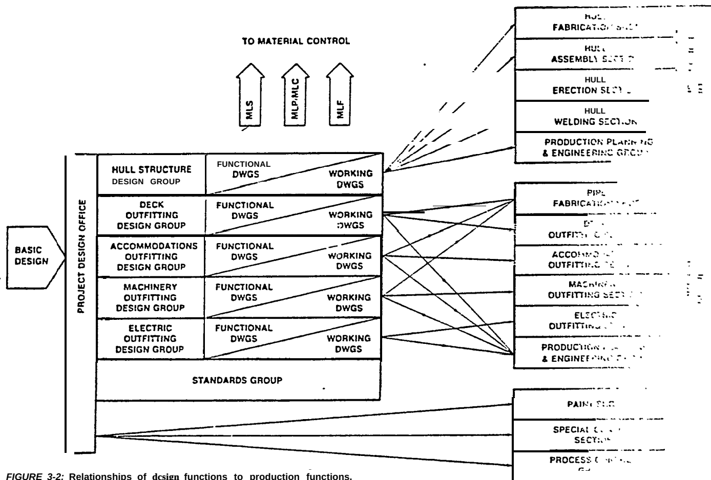
FIGURE 3-2: Relationships of design functions to production functions.
