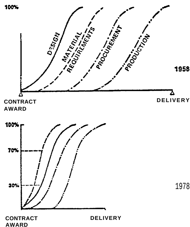
FIGURE 1-1 Overlap of outfit design, material definition, procurement and production which has been achieved by the most competitive shipbuilders. When only 30% of a design is completed, 70% of its required material is defined.
