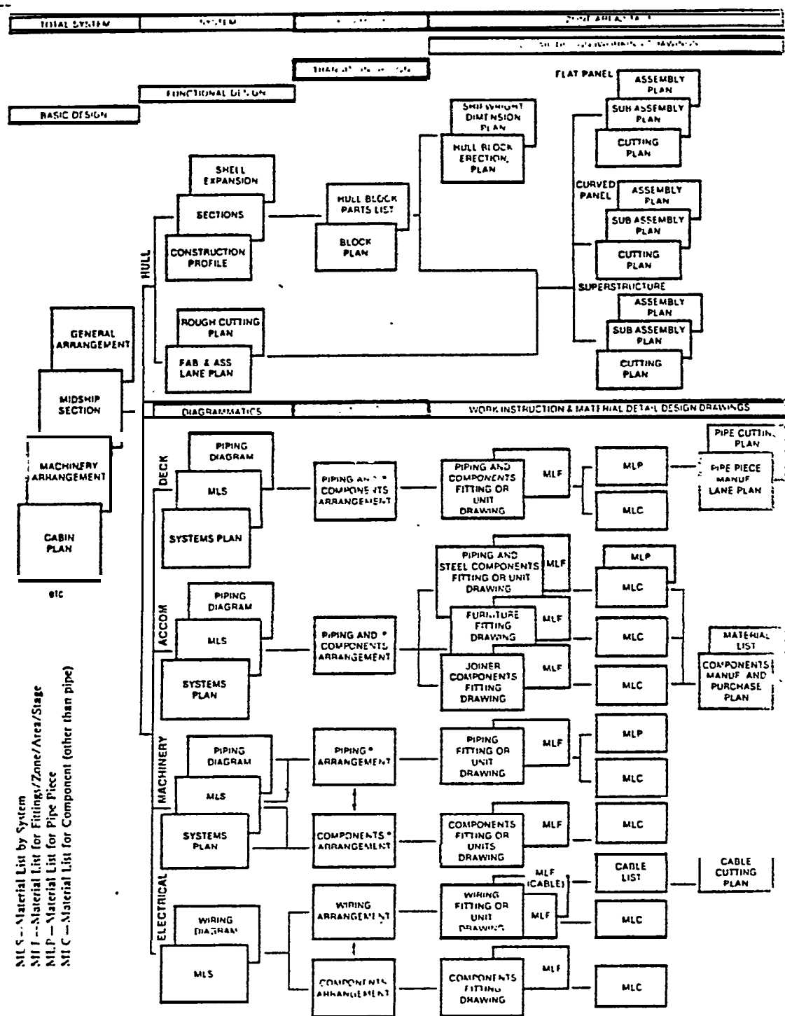
FIGURE 2-2 Product-oriented Design Process. Transition Design introduces zones and interrelations with systems. The items marked “***” are sometimes freehand. But, they are sufficient for quickly conveying arrangements and system/zone relationships to detail designers. The latter refine arrangements, a decisive stage during preparation of work instruction and material detail-design drawings.
