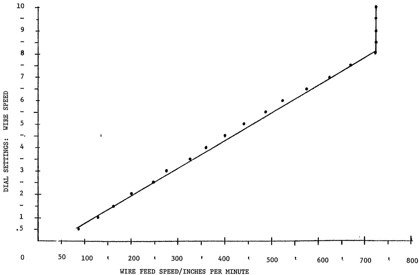
WIRE FEED SPEED VS. DIAL SETTINGS 3/64" DIAMETER 5556 ALUMINUM ALLOY FILLER WIRE AIRCO SYSTEM 1 FEEDER; AIRCOMATIC GUN: MANUAL MODE
