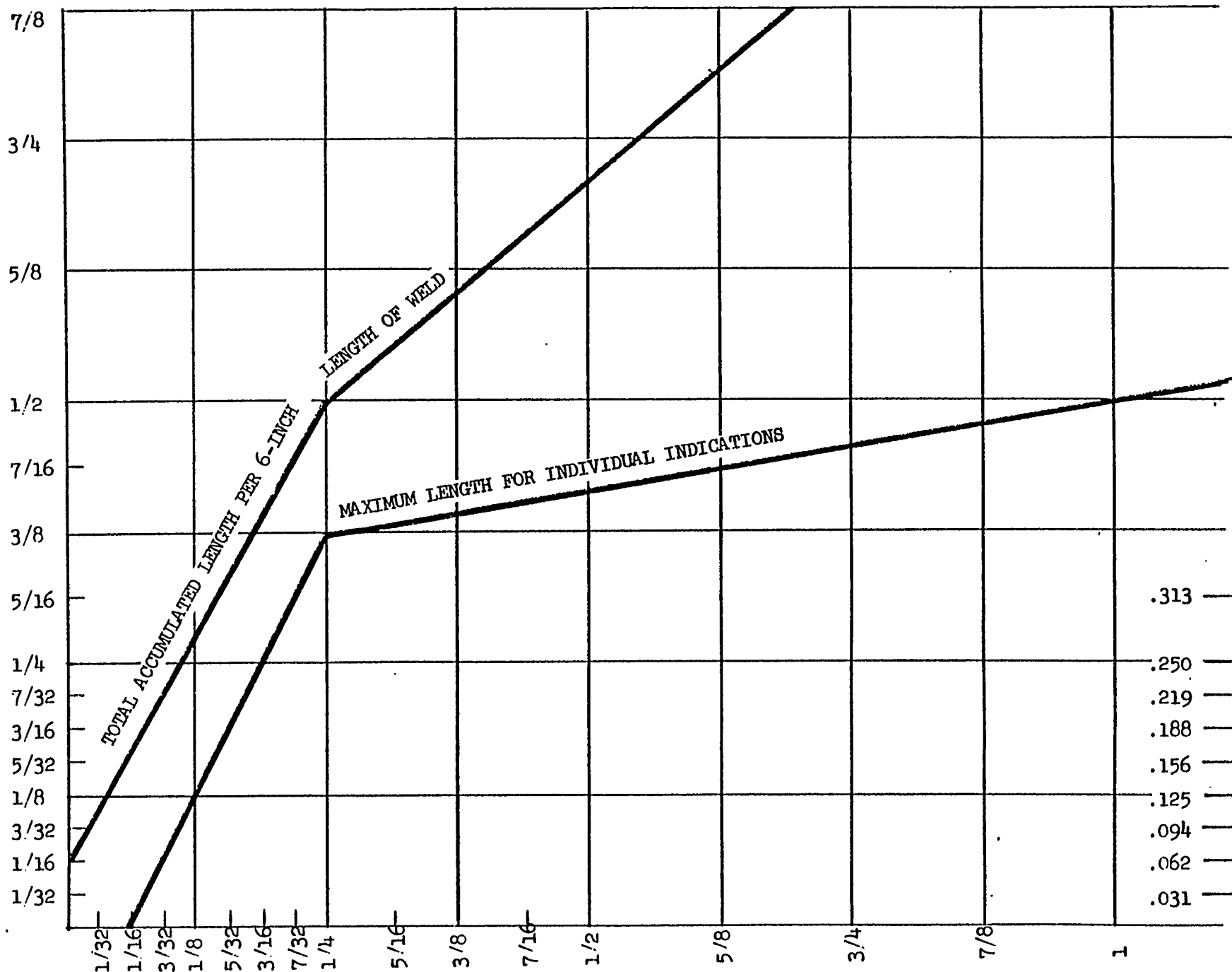
DESIGN MATERIAL THICKNESS "T" IN INCHES NAVSHIPS 0900-003-9000 - CLASS 3 SLAG (INCLUSIONS)
