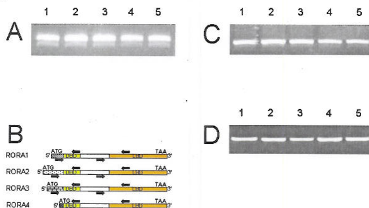
Figure 2 The transcriptional level of RORA and its isoforms in various normal tissues. Lane 1 brain; Lane 2 breast; Lane 3 liver; Lane 4 ovary; Lane 5 prostate. Total RNA was prepared from normal human tissues and cDNA was generated. Semi-quantitative RT-PCR was performed using the universal primers for all RORA isoforms and the specific primers for each isoform to measure the level of RORA. A. RORA universal primers; B. A schematic diagram showing the four different isoforms of RORA. The bold arrows show the positions of specific primers for each isoform and the universal primers for all isoforms. DBD DNA binding domain; LBD ligand binding domain. C. RORA1 (isoform 1) primers; D. RORA4 (isoform 4) primers.
