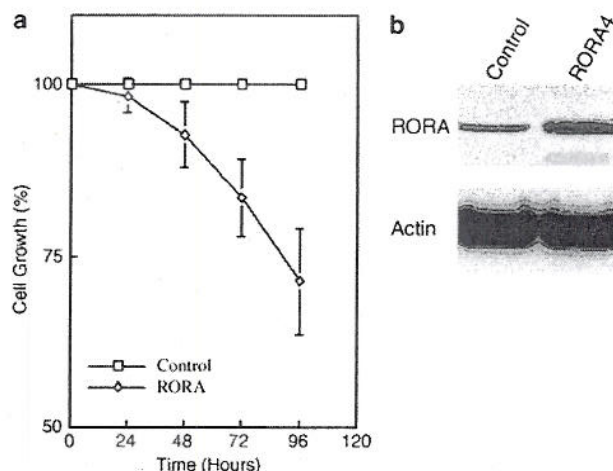
Figure 6 Effect of RORA overexpression on cellular growth. (a) MCF12F cells were plated and incubated overnight before transfection. The plasmids (pcDNA3 as control and pcDNA3-RORA4) were transfected into cells using a Lipofectamine 2000 transfection kit following the manufacturer's protocol. The cell number was counted 24, 48, 72 and 96 h later. All results are the average of at least three independent experiments with s.d. shown by bars. (b) The level of RORA in pcDNA3-RORA4 transfectants detected by the Western blotting assay. Top row RORA; and bottom row actin.
