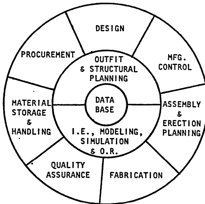
Figure 13. Shipyard activity wheel. A common or central data base can provide the support necessary for an integrated approach to all the activities of a manufacturing concern. For a shipbuilder, outfit and structural planning are key tasks with overall support from industrial, manufacturing, and systems engineering and their associated tools of simulation, modeling, and operations research. Planning and engineering provide the basis by which the actual or physical "doing" of ship production is accomplished (the seven outer tasks). Information and communication provide means by which all decisions are made and therefore represents the core or cornerstone of an effective organization.
