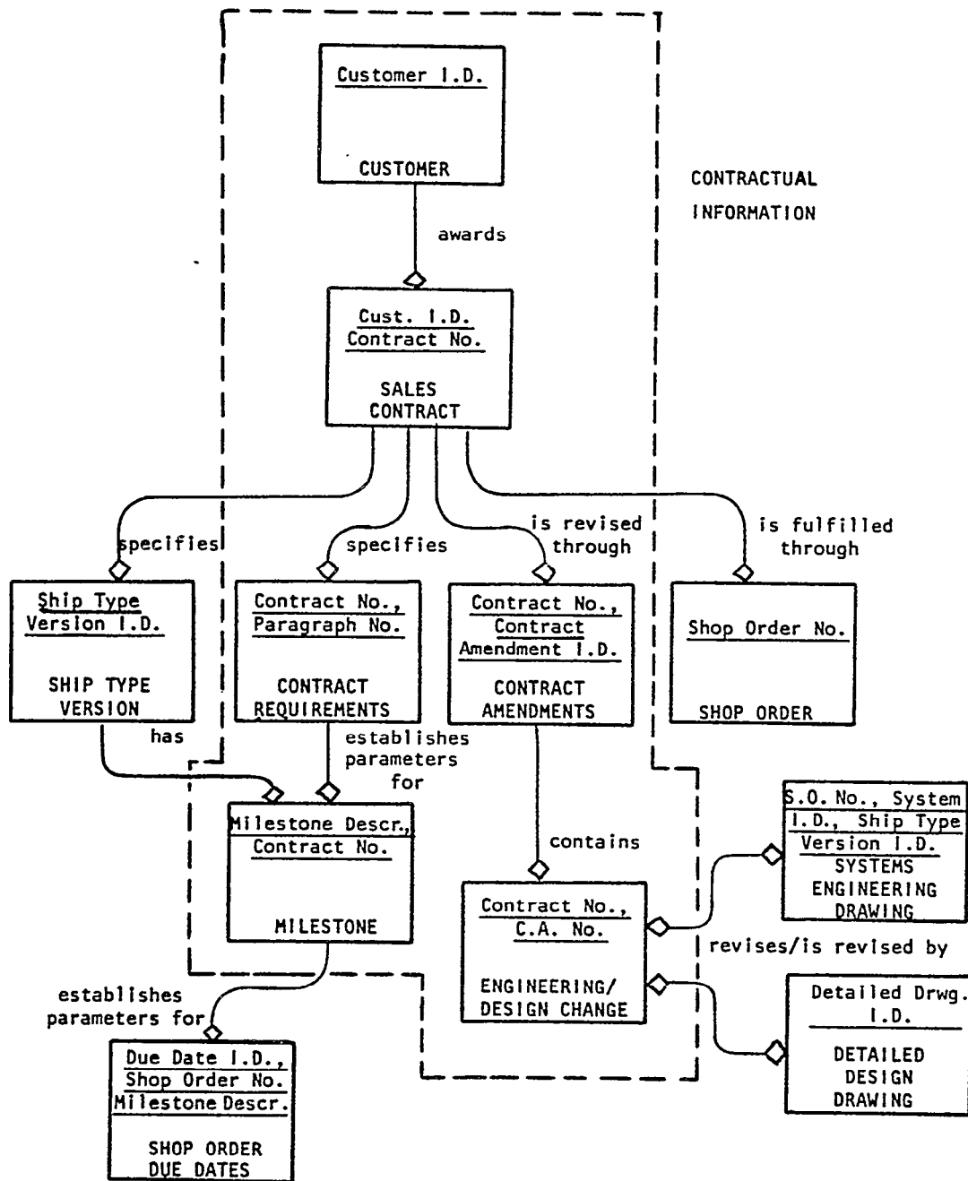
Figure 4. Contractual information needed to support outfit planning. A customer awards 0, 1, or many sales contracts. Each sales contract specifies 0, 1, or many ship-type versions and contract requirements. A sales contract is revised through 0, 1, or many contract amendments and is fulfilled through many fabrication and assembly shop orders. A contract requirement establishes parameters for 0, 1, or many milestones which, in turn, establish parameters for many shop order due dates. A contract amendment contains 0, 1, or many engineering/design changes. A systems engineering and detailed design drawing is revised by 0, 1, or many of these engineering/design changes.
