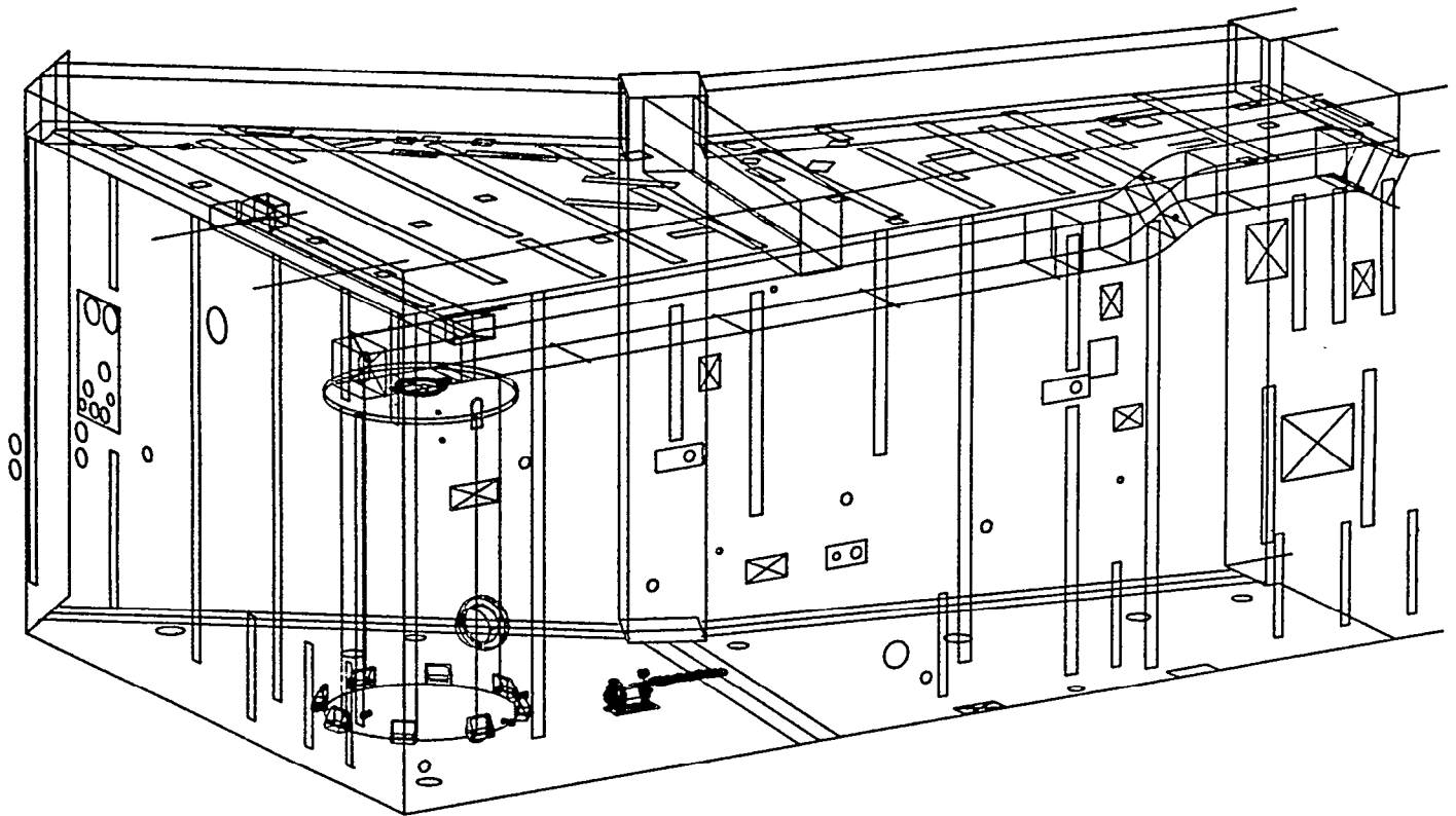
Figure 5. Heating, Ventilating, and Airconditioning Ducts
