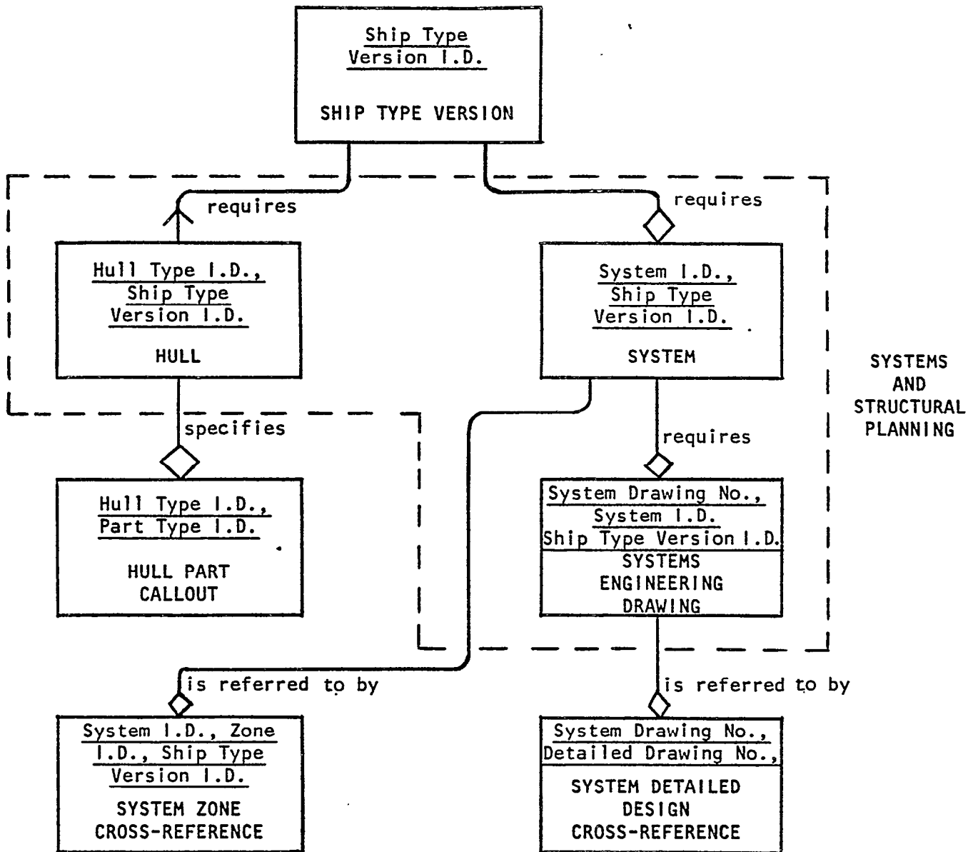
Figure 6. Systems and structural information necessary to support outfit planning. A ship type version requires zero or one hull type and requires zero, one, or many systems. A system (i.e., piping, electrical) requires zero, one, or many systems engineering drawings to describe it. For transition design the systems engineering drawings are referred to by zero, one, or many system-zone and system-detailed design cross-references.
