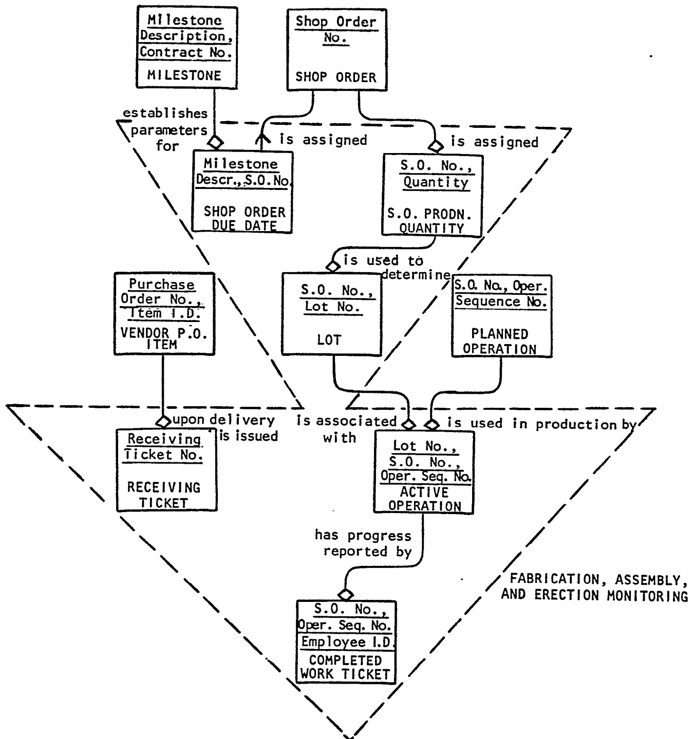
Figure 10. Fabrication, assembly, and erection monitoring which supports control necessary for outfit planning. A shop order is assigned a due date based on parameters set forth in a milestone. The milestone due data determines several shop order due dates. A shop order is assigned one or more production quantities (depending on whether it is a part or pallet S.O.) which in turn are broken down into one or more lots. A planned operation is used in production by zero, one, or many active operations, and each active operation is associated to a lot number with any particular shop order. The status of an active operation is usually reported by several completed work tickets. Procured materials are similarly accounted for by a receiving ticket.
