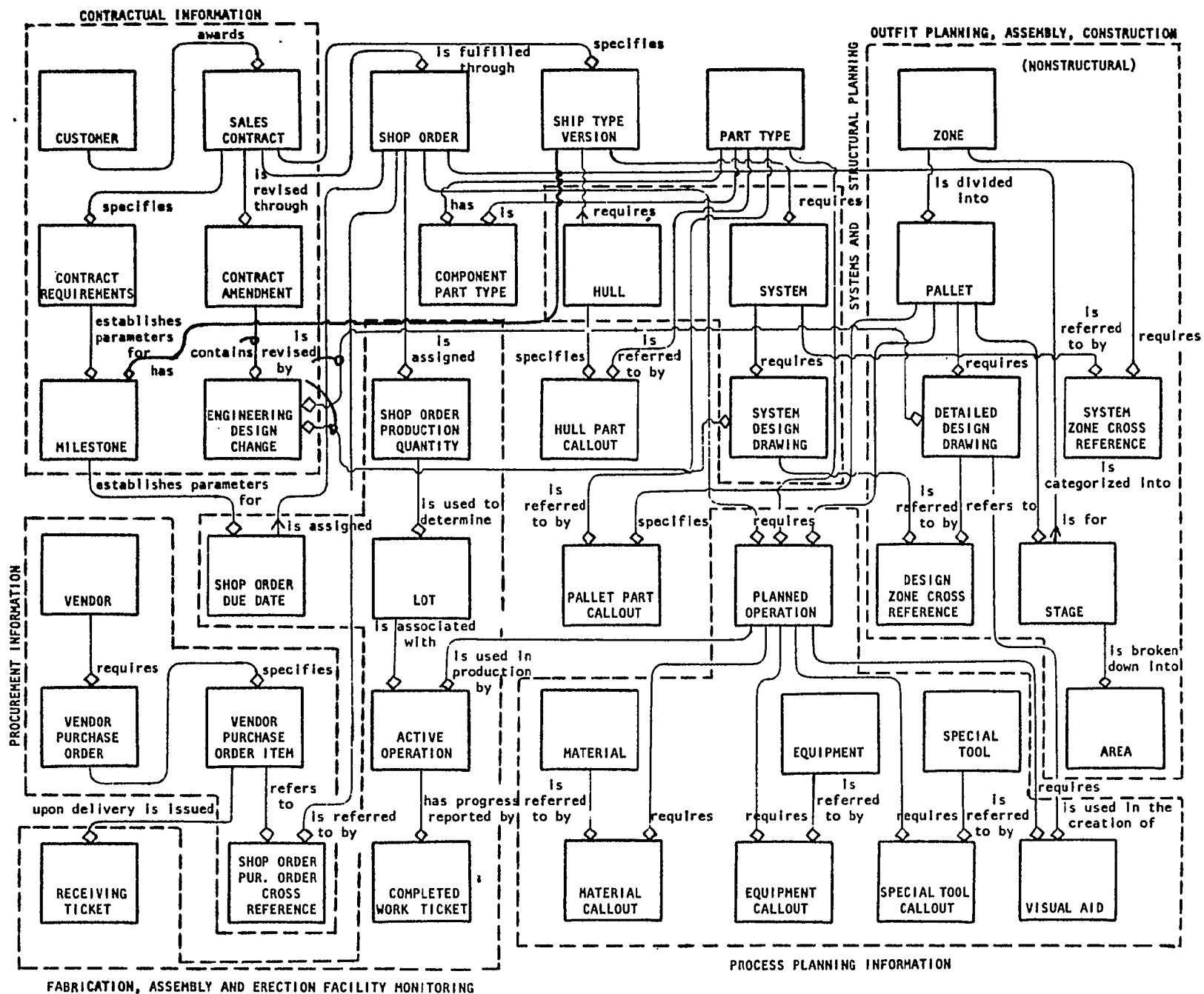
Figure 12. Overall conceptual design of a data base model for outfit planning.
