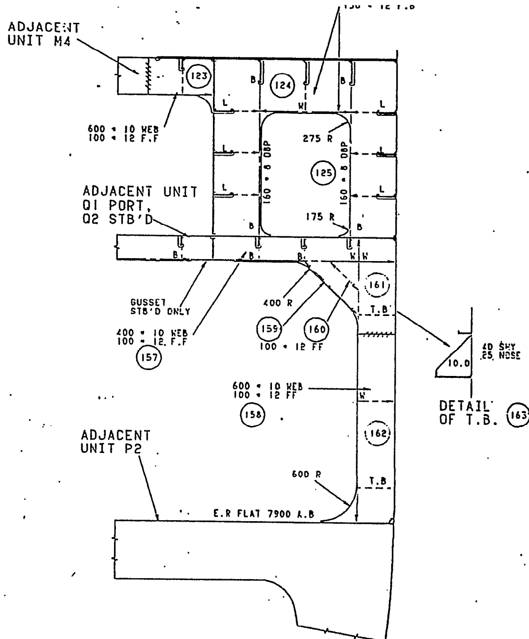
SECTION AT WEB 71
