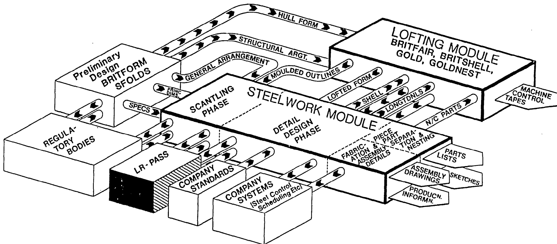
Fig.1 BRITSHIPS 2 INFORMATION FLOW
