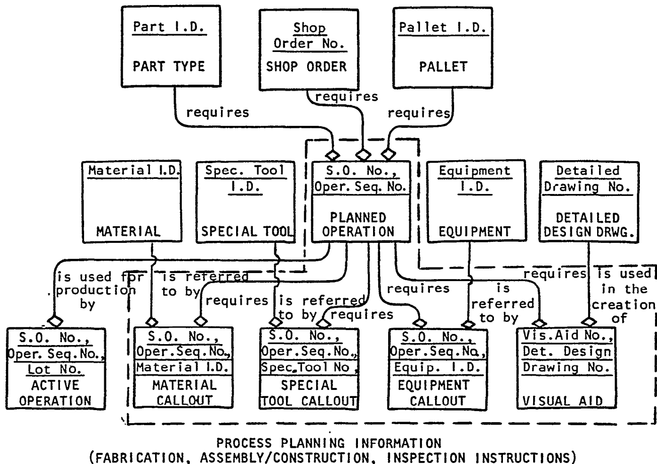
Figure 8. Process planning information necessary to support outfit planning. There are two types of process plans, fabrication of a part and assembly of a pallet, each requiring the same type of process planning information. A shop order is either for part fabrication or pallet assembly (pre-outfitting) and requires therefore zero, one, or many planned operations. A part, then, requires zero, one, or many planned operations or a pallet requires zero-one, or many planned operations depending on the shop order type. A planned operation requires zero, one, or many material callouts, special tool callouts, equipment callouts, and visual aids, and is used for production by zero, one, or many active operations.
