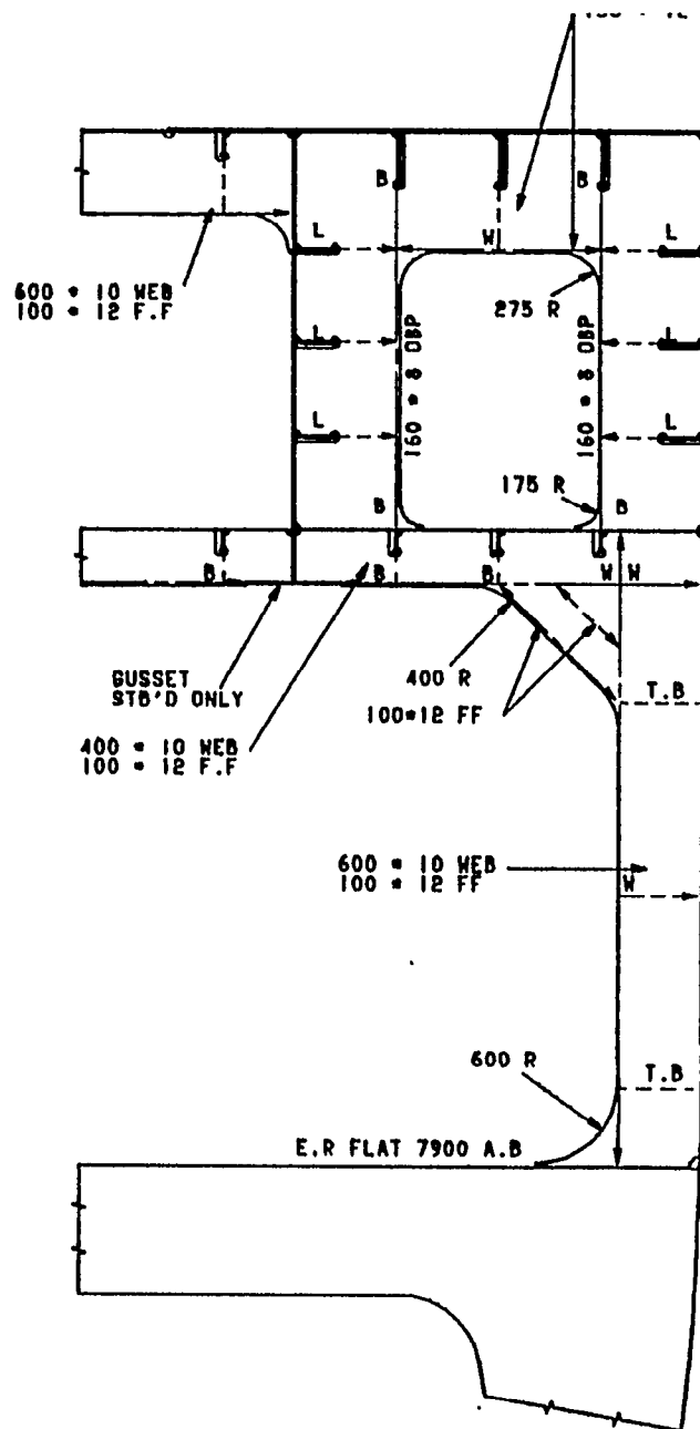
SECTION AT WEB 71
