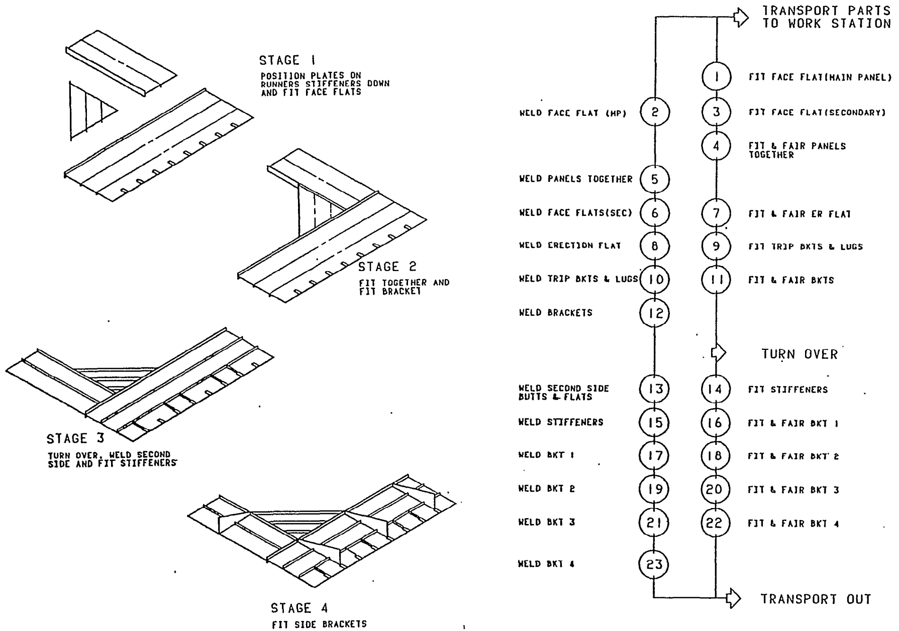
Fig.16 ASSEMBLY SEQUENCE AND PREFERRED PROCESS FLOW CHART
