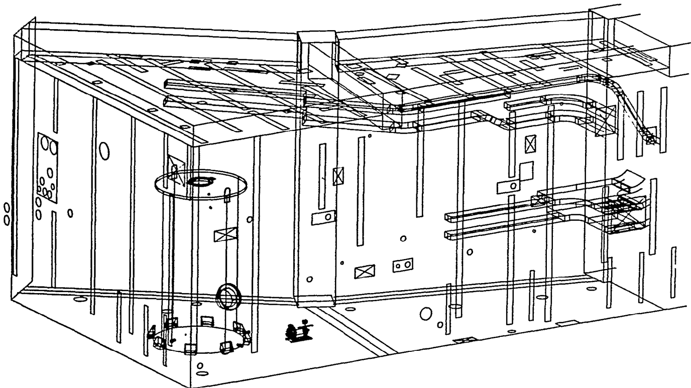
Figure 4. Electrical Raceways
