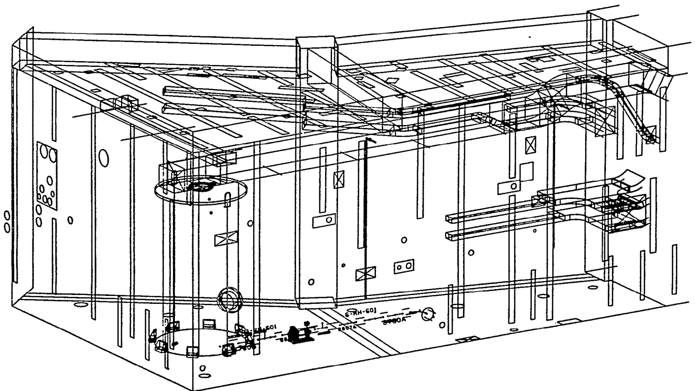
Figure 6. Cubicle 18 (Piping and Supports Added)
