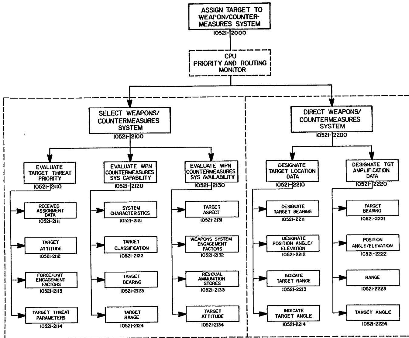
STAGE IDENTIFICATION DIAGRAM - FUNCTIONAL ANALYSIS RESULTS
