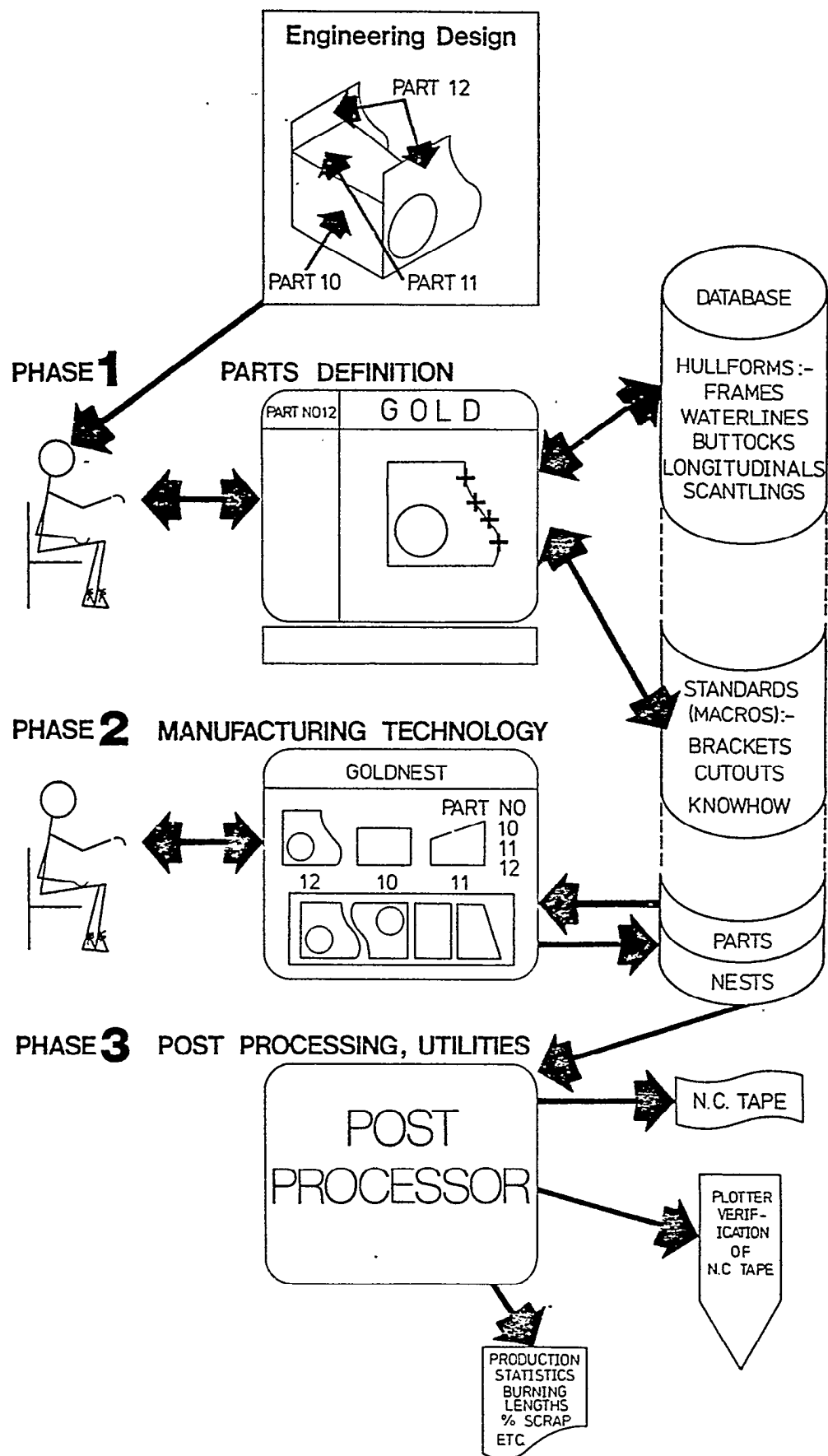
Fig.1 9 INFORMATION FLOW THROUGH GOLD
