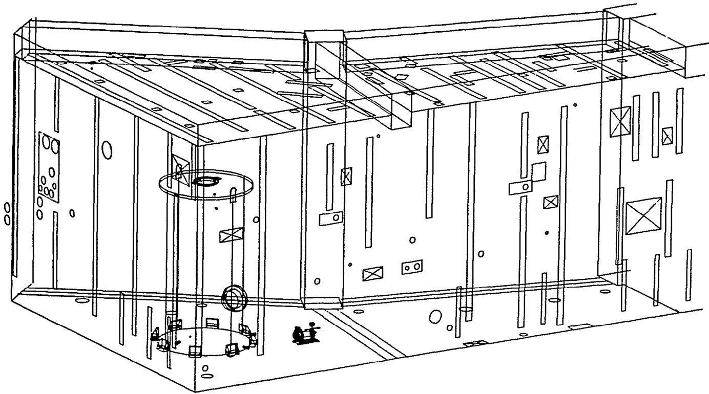
Figure 3. Building, Structure, Penetrations, and Equipment
