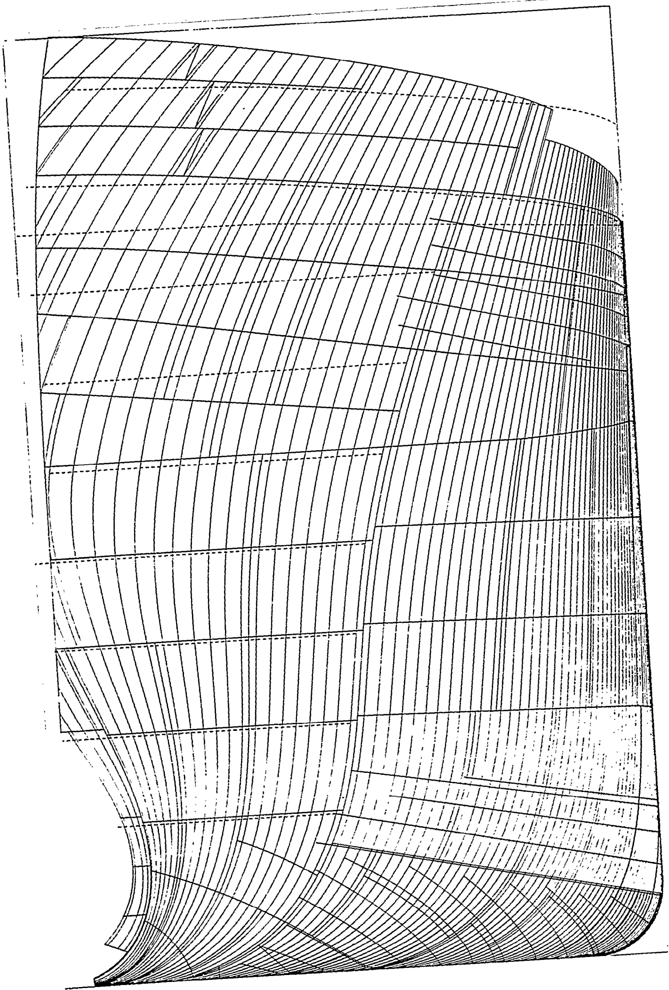
Fig.9 SHELL ARRANGEMENT LONGITUDINALS AND DECK-AT-SIDE LINES AS DEFINED IN THREE DIMENSIONS
