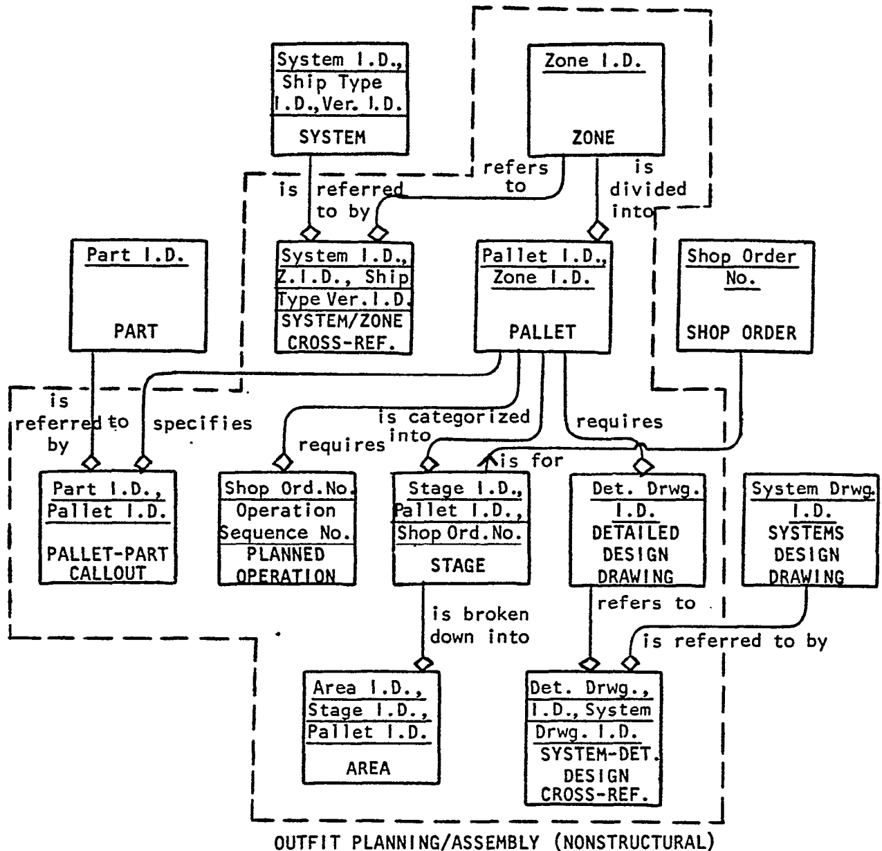
Figure 7. Outfit planning/assembly information. A zone is divided into zero, one, or many pallets, and a zone can refer to zero, one, or many system-zone cross-references (in other words, a zone has several systems running through it). A pallet is categorized into zero, one, or many stages which, in turn, are broken down into area categories. A pallet also requires zero, one, or many detailed design drawings (which refer to systems drawings). A pallet requires zero, one, or many planned operations for assembly and specifies zero, one, or many parts of which it is comprised.
