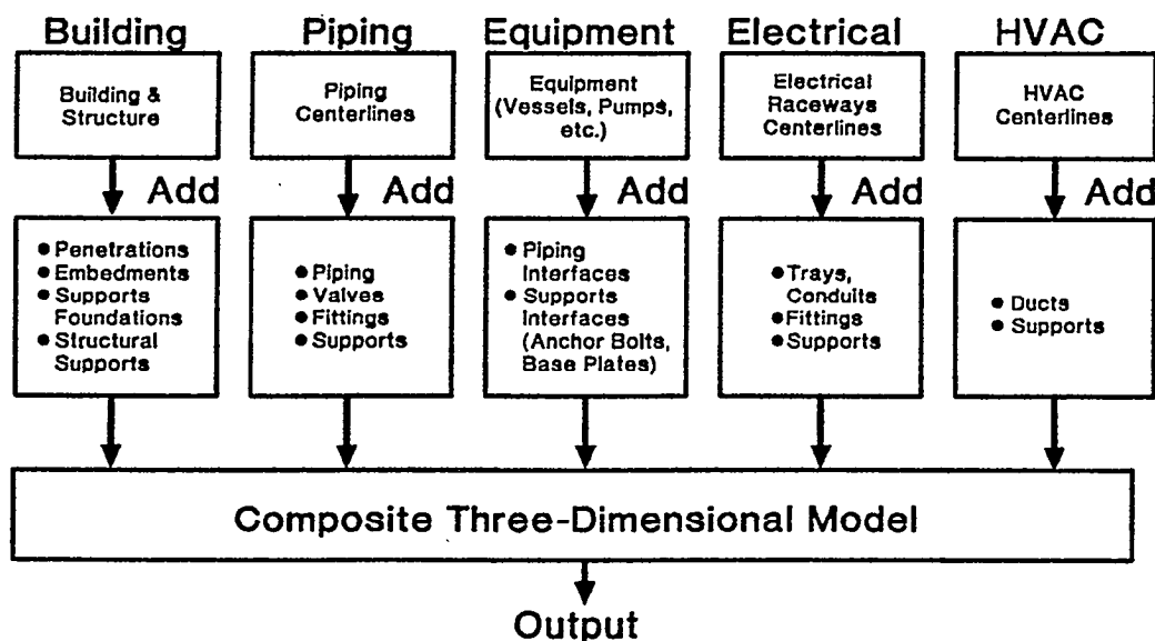
Figure 2. Layer Technique for Generating Plant Model
