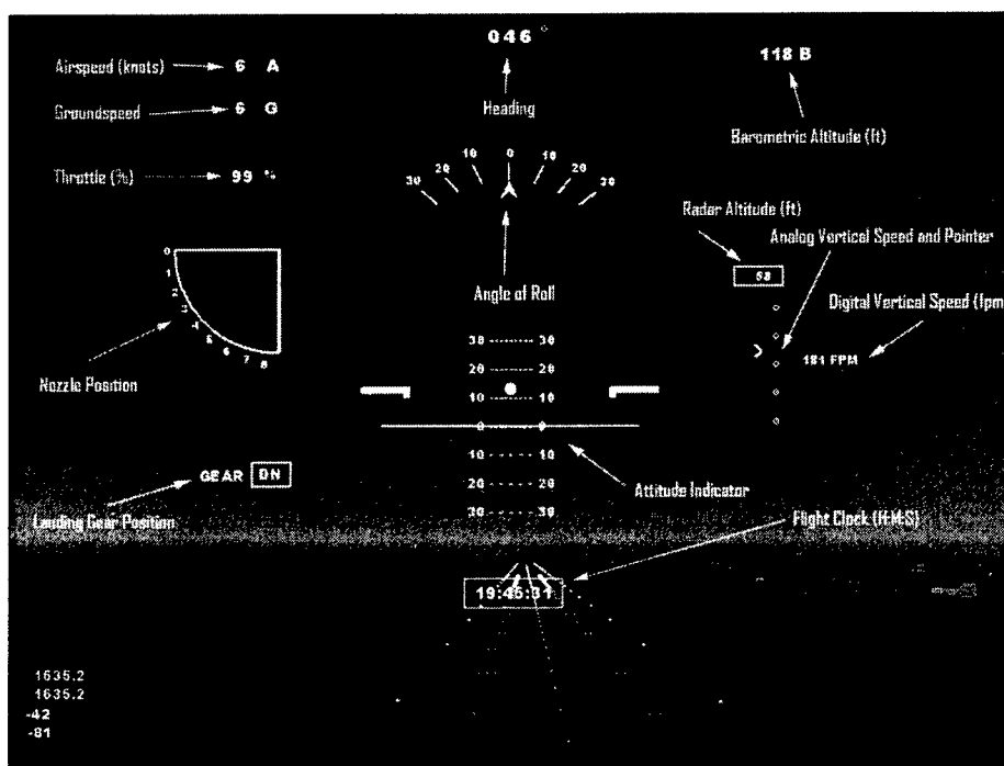
Figure 5-4: Harrier Conventional Head-Up Display
