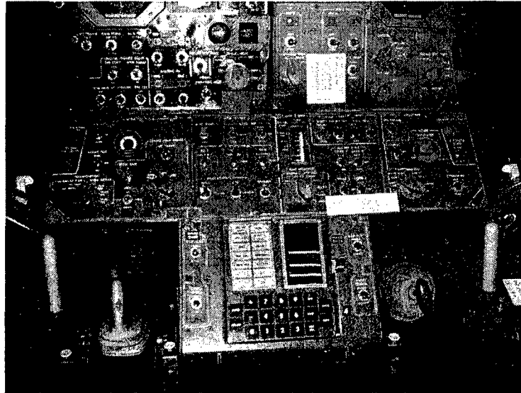
Figure 2-1: Apollo Lunar Module Cockpit (from [19])
