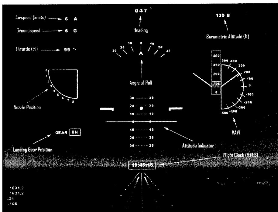
Figure 5-3: Harrier Head-Up Display with VAVI Display
