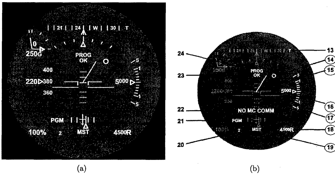
Figure 2-8: MV-22 Osprey Hover Mode HUD (from [25])
