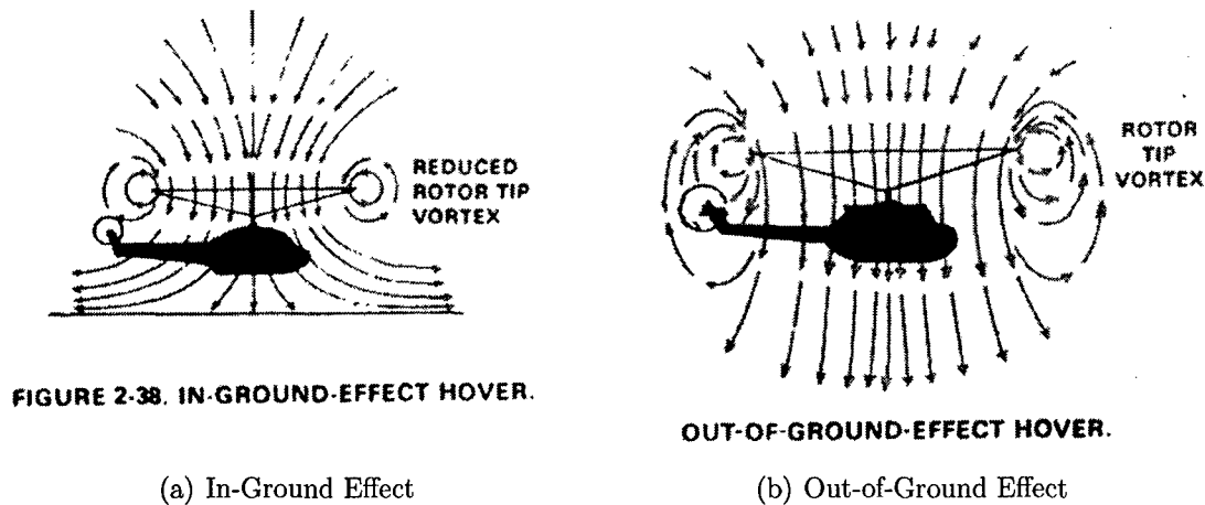
Figure 1-2: Ground Effect(from [6])
