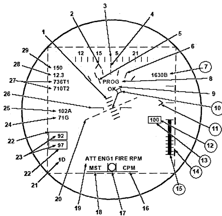
Figure 2-5: UH-60 Black Hawk HUD (from [23])
