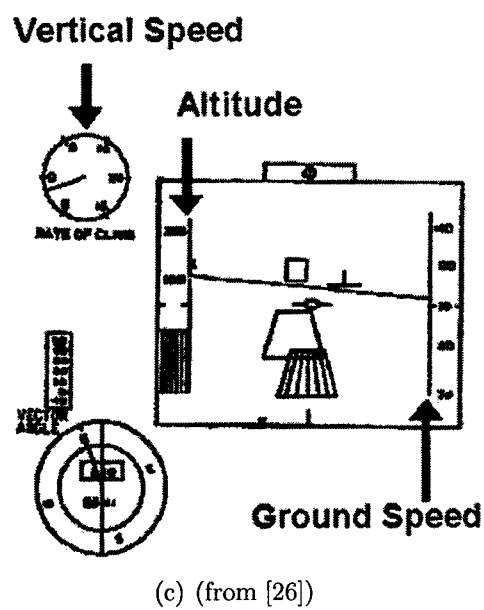
Figure 2-9: Proposed V/STOL Displays
