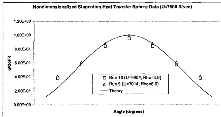
Figure 18 Comparison between Heat Transfer Measurements around a Hemispherical Nostetip and Fay Riddell Predictions (U = 7,000 ft/s)
