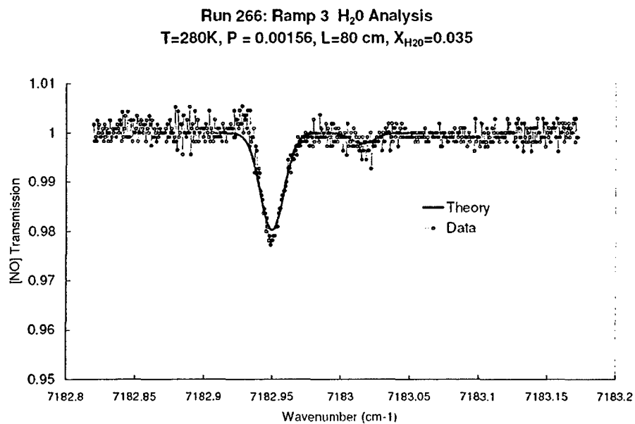
Figure 30 \text{H}_2\text{O} line Shape Measurement of the Freestream for Run 266. The Temperature of the \text{H}_2\text{O} was Determined to be 280°K
