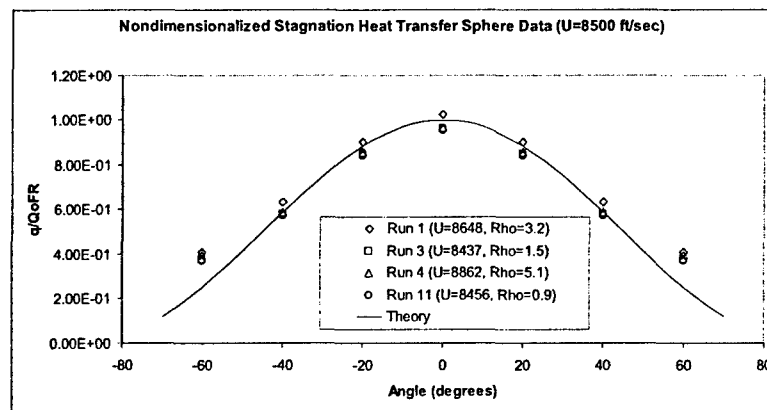
Figure 20 Comparison between Heat Transfer Measurements around a Hemispherical Nostetip and Fay Riddell Predictions (U = 8,500 ft/sec)
