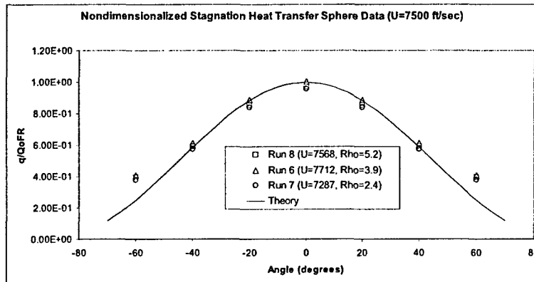
Figure 19 Comparison between Heat Transfer Measurements around a Hemispherical Nostetip and Fay Riddell Predictions (U = 7,500 ft/sec)
