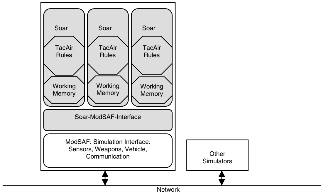
Figure 1: System organization for TacAir-Soar
