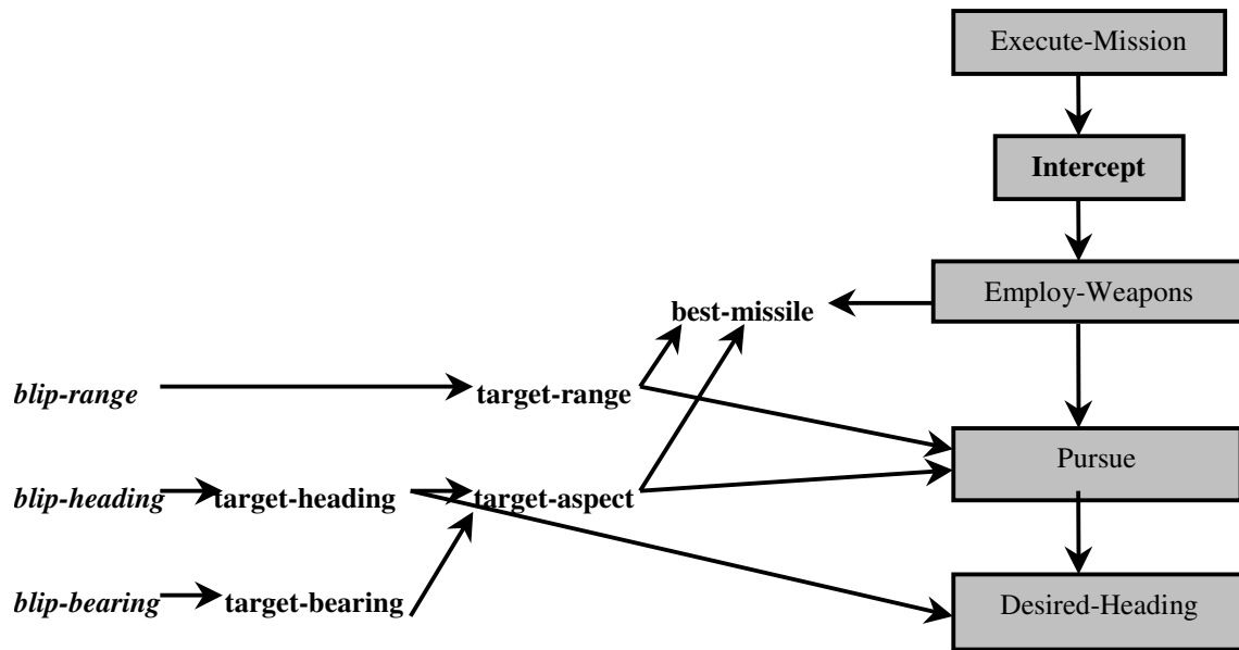
Figure 4: TacAir-Soar changes the goal hierarchy in response to changes in the situation-representation hierarchy (and vice versa)
