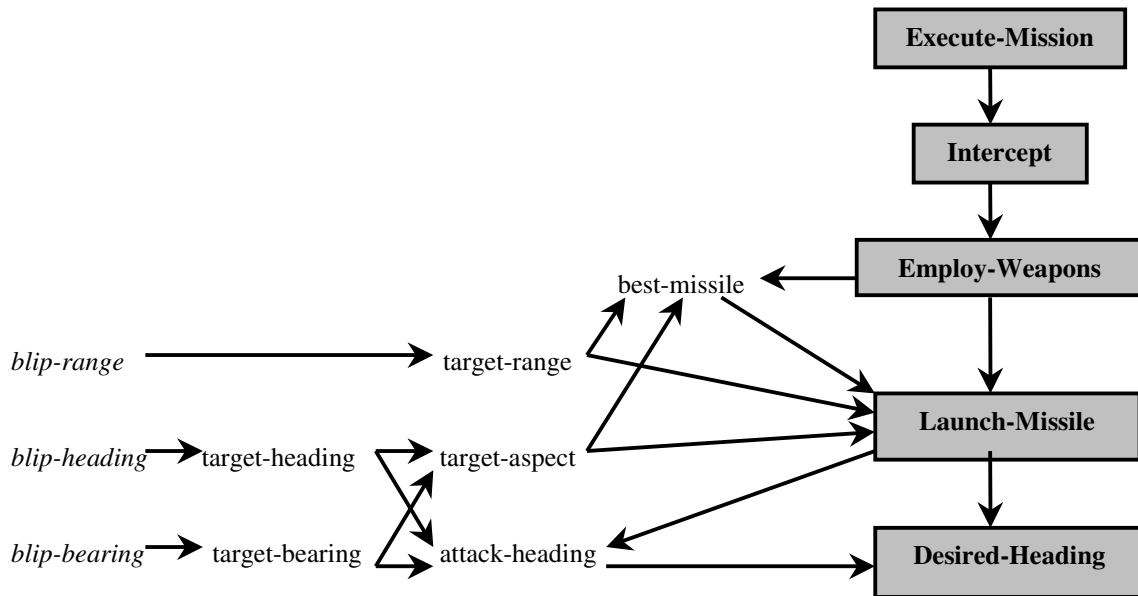
Figure 3: Sample active goal and situation hierarchies
