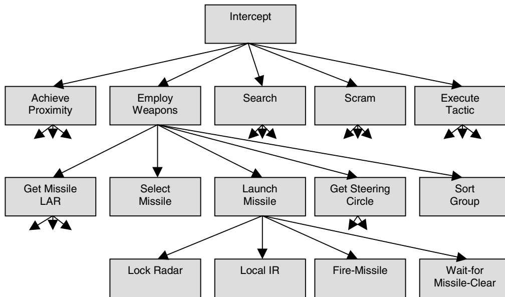
Figure 2: Example operator hierarchy decomposition
