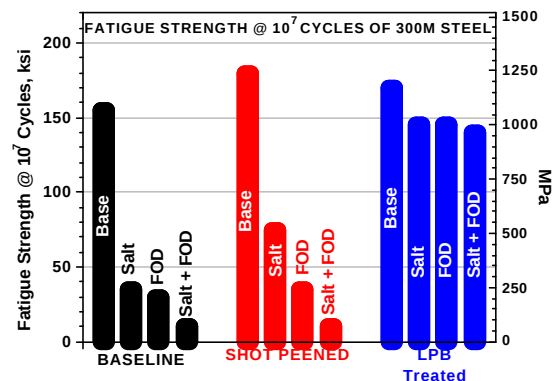
FIGURE 11 – Summary of Fatigue Results
