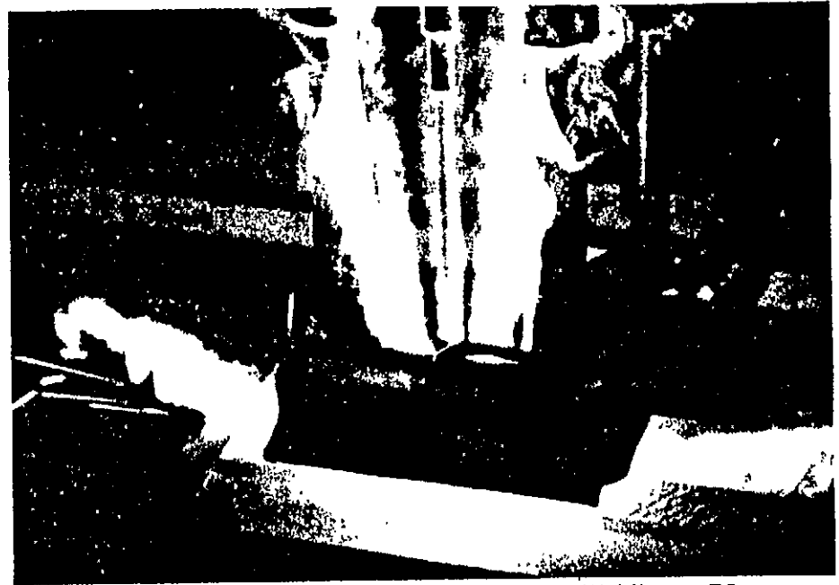
Eccentric Spinning Wire Method Narrow Gap Welding 79
