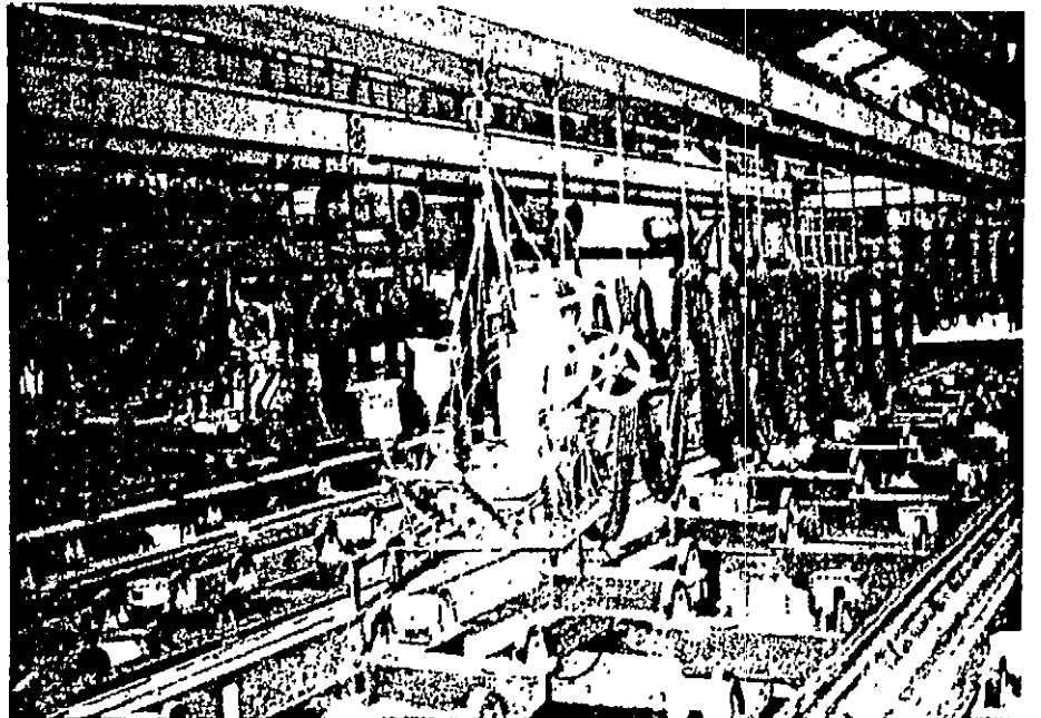
One Side Welding Stations
