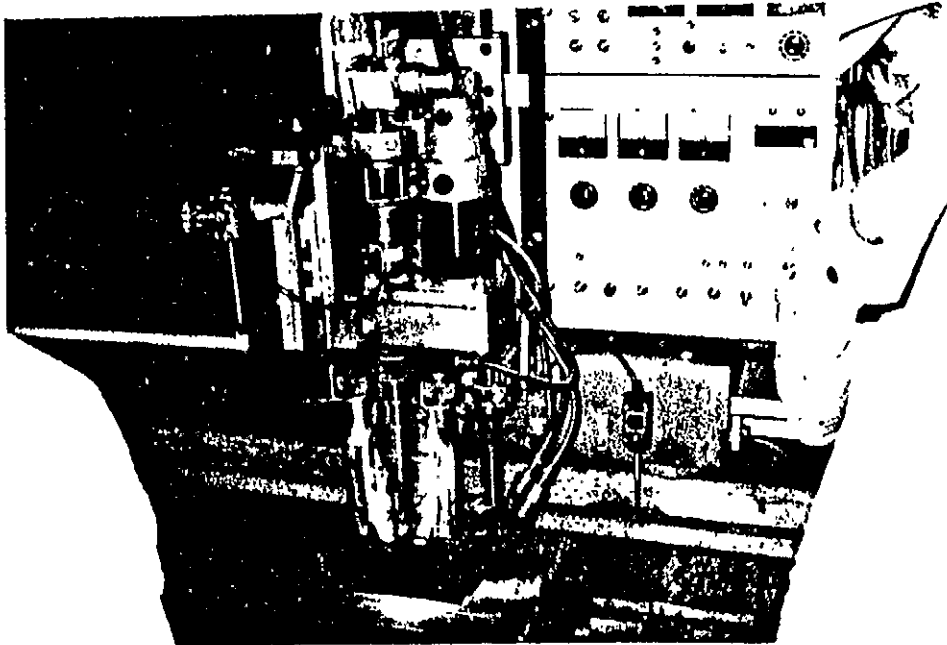
Eccentric Spinning Wire Method Narrow Gap Welding 78
