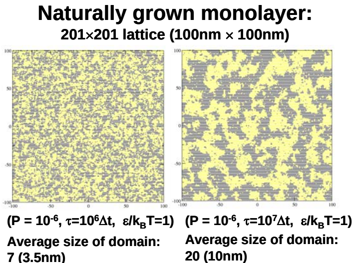
Figure 37. Dependence of domain size on chemisorption rate \tau^{-1}
