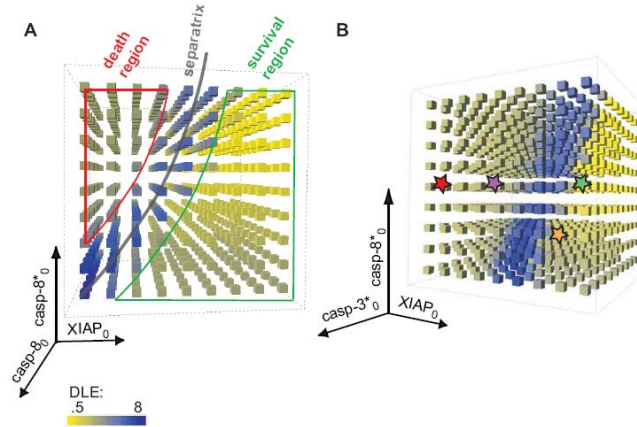
Figure 6: An LCS (stable manifold) separating the phases space of a cell model into death and survival regions.
