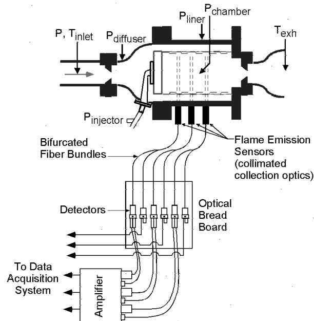
Figure 6. Instrumentation for combustion dynamics experiments.
