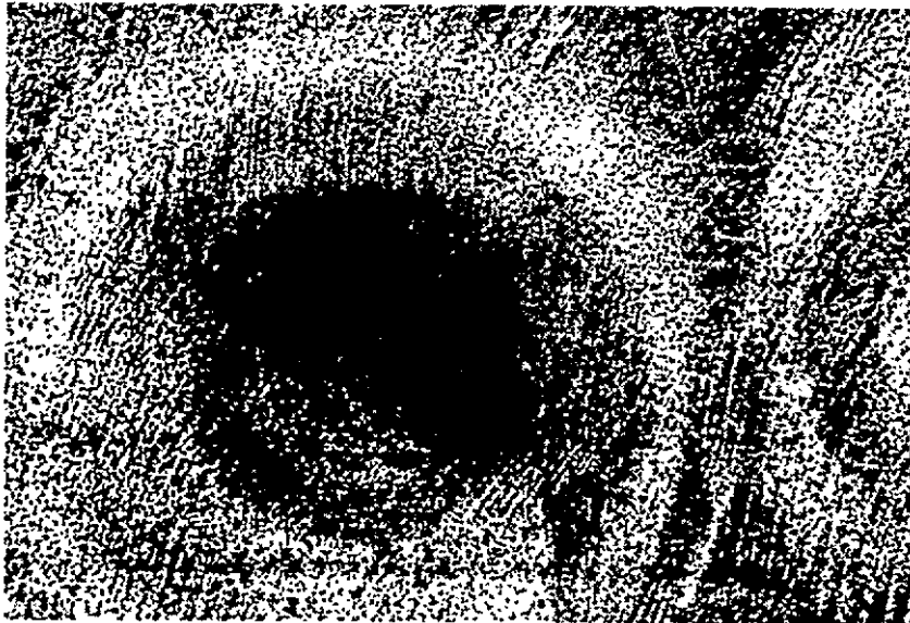
Photographic Standard No. 10 Disc Sanding and/or Power Brushing to Burnt Areas where Zinc Epoxy Primer has been applied as Shop Primer.
