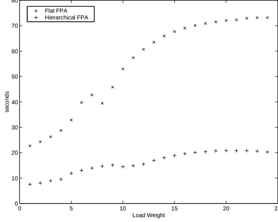
Figure 3.3: Run time vs. traffic load.
