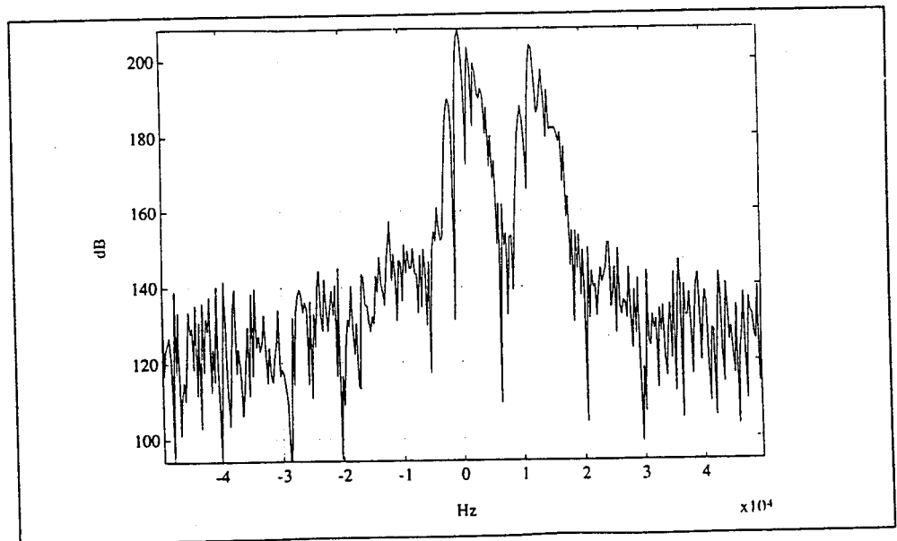
Figure 2.5: Power spectrum of reflected return signal
