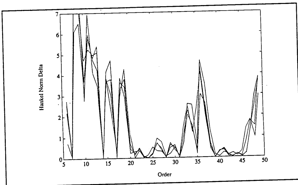
Figure 5.29: Upper Bound of Cauchy Sequence for Hankel Norm of Truncated MME Hankel Operator Day91010
