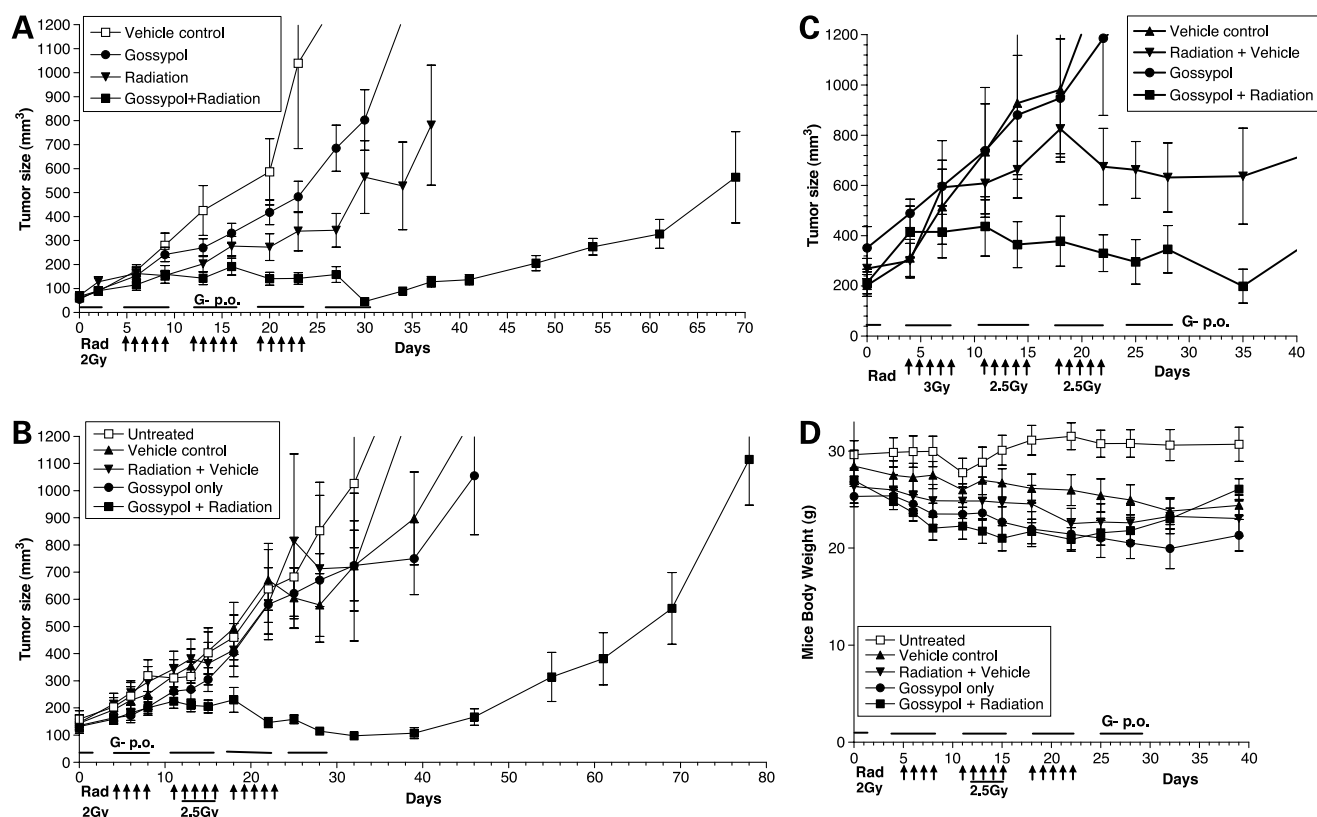
Figure 3. (–)Gossypol [G(–)] in combination with radiation achieves tumor regression in androgen-independent prostate cancer PC-3 xenograft model. PC-3 xenograft tumor growth curves after treatment with fractionated X-ray irradiation and G(–), alone or in combination, where the tumor sizes at the start of G(–) treatment are around 75 mm 3 (A), 150 mm 3 (B), and 230 mm 3 (C). PC-3 cells ( 5 \times 10^6 ) were s.c. injected into the lower back above the tail of each mouse, both sides. When tumors reached appropriate size, the mice were randomized into five to eight mice per group and treated with either G(–) 10 mg/kg p.o., q.d. \times 5 , \times 4 weeks; or X-ray irradiation 2 to 3 Gy, q.d. \times 5 , \times 3 weeks, or their combination. Vehicle control group and radiation only group received same amount of 10% ethanol which is solvent for G(–). The average tumor sizes were shown ( n = 10-16 ). The total radiation doses were 30 Gy for A and B, and 40 Gy for C. D, mice body weights from experiment B during treatment were plotted. (–)Gossypol in combination with radiation seems not to have significant toxicity as compared with either treatment alone or vehicle control.
