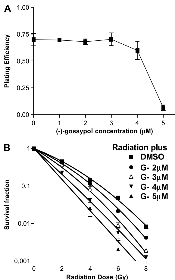
Figure 1. Clonogenic assay of PC-3 cells exposed to X-ray irradiation with or without (–)-gossypol [G(–)]. PC-3 cells were plated in 6-well plates and G(–) or DMSO vehicle control were added. Then cells were irradiated with X-ray, 300 kV, dose rate \sim 3 Gy/min at room temperature with doses up to 8 Gy. The plates were cultured for 12 d, stained with crystal violet, and the colonies with over 50 cells were counted with ColCount colony counter. The survival curves were plotted with linear-quadratic model. A , plating efficiency (survival fraction) of G(–) treatment alone. B , clonogenic survival curves of PC-3 cells in response to irradiation [normalized for the killing of G(–)].
