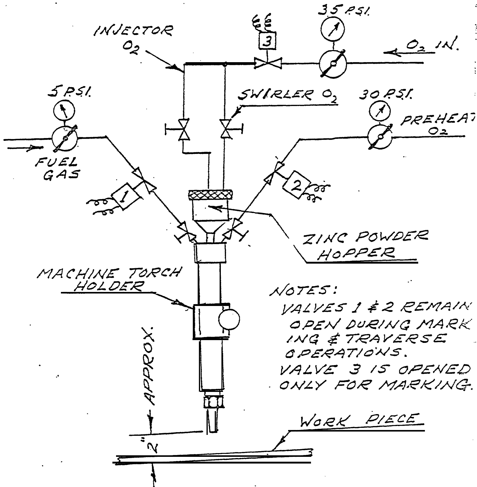
TYPICAL POWDER MARKING TORCH ARRANGEMENT FOR PROGRAMMED PLATE MARKING.
