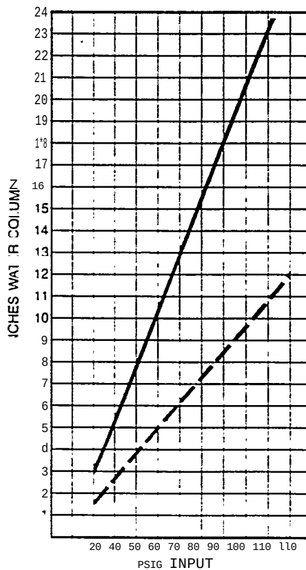
913/953 Transvector
