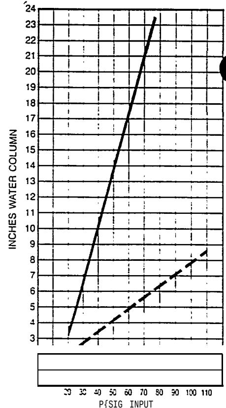
914/954 Transvector
