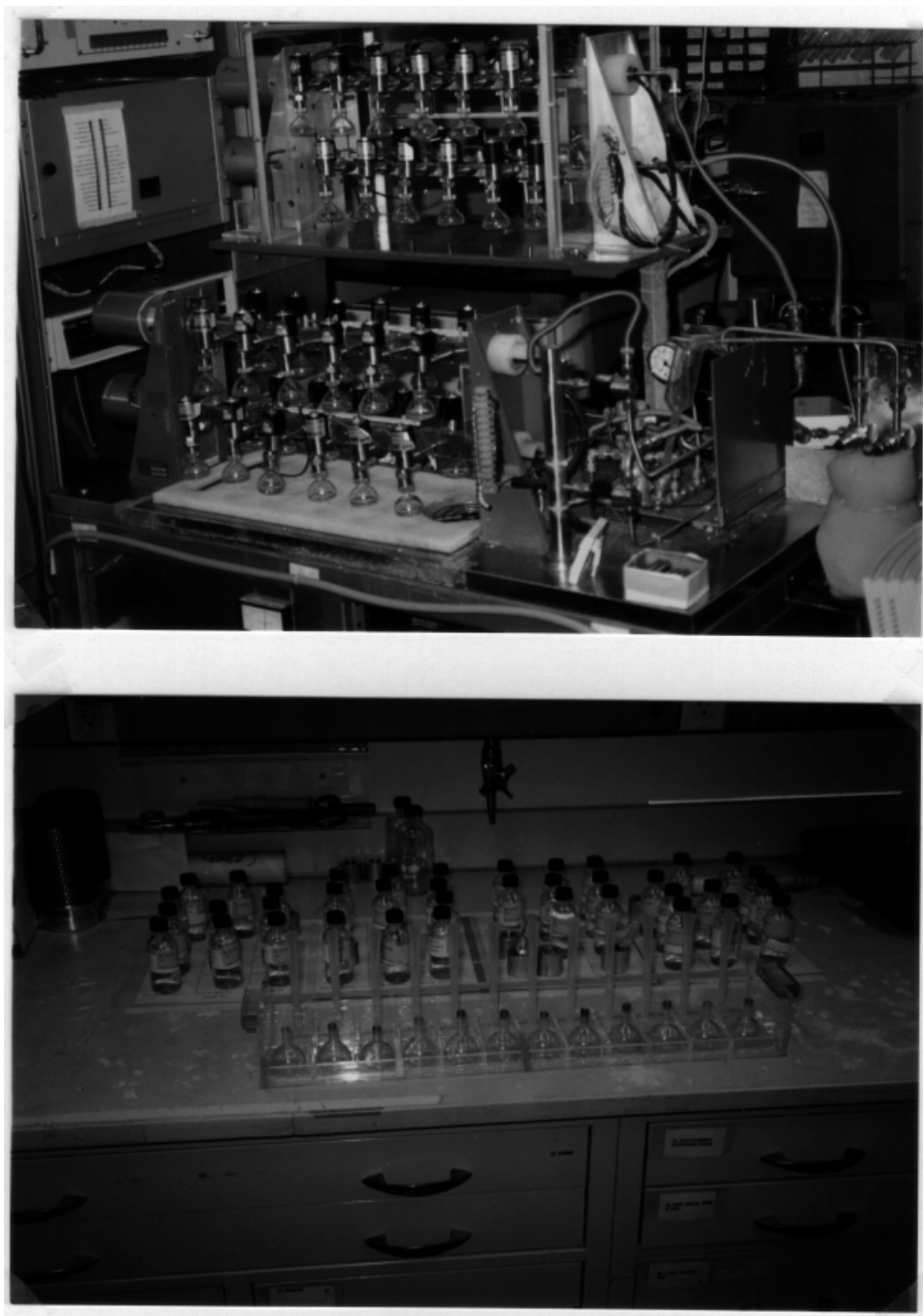
Fig. 30. (a) Micromass CO 2 -H 2 O equilibration system in author's laboratory. (b) Template for this system set up with 48 samples.
