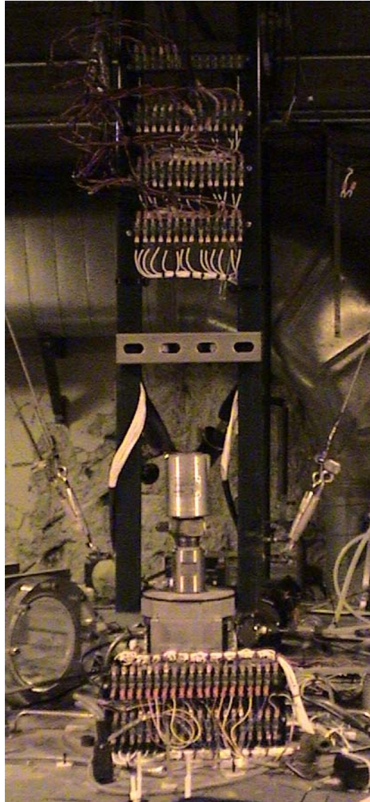
Figure 1.1. Updated wiring on the centrifuge table.
