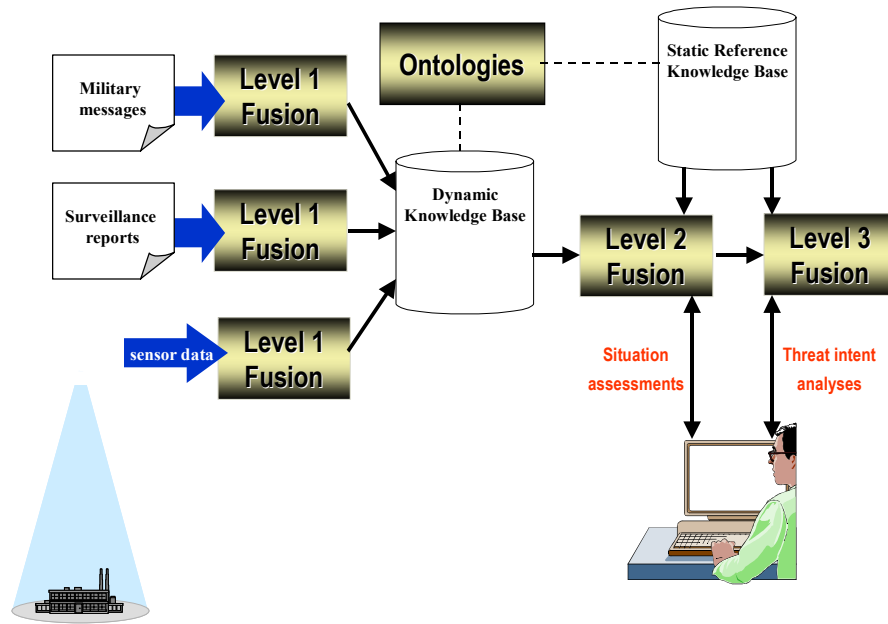
Figure 2: Ontology-based Fusion Architecture
