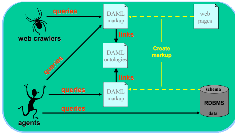
Figure 1 – DAML markup for artifacts such as web pages, database schemas, legacy software interfaces, and sensor outputs.
