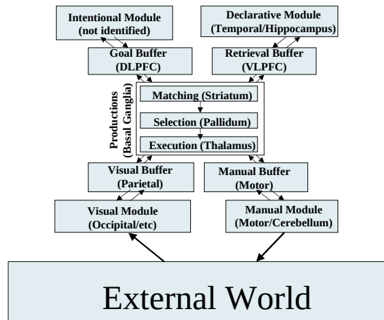
Figure 1: ACT-R Architecture, including mapping of ACT-R components to brain regions.
