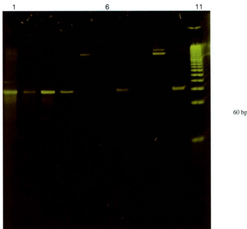
Figure 8 Visualization of the ssDNA products with Sybr Gold on a PAGE gel. As a control, samples of the ssDNA library (lane 1, 120 ng; lane 2, 12 ng) and the selected ssDNA sequence (lane 3, 120 ng; lane 4, 12 ng) are provided. The ssDNA that was originally coupled to the magnetic beads is shown in lane 5 (DNA library), lane 6 (blanc to which no DNA was added) and in lane 9 (selected sequence). The ssDNA that was originally not couples to the magnetic beads can be found in lane 7 (DNA library), lane 8 (blanc to which no DNA was added) and in lane 10 (selected sequence). Lane 11 is the Super-ladder-Low 20bp Ladder (50 bands: 20bp-1000bp in exact 20bp increments, brighter bands at 200bp and 500bp).
