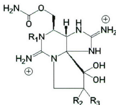
Figure 9 Saxitoxin, paralytic shellfish toxin produced or elaborated by planktonic algae (dinoflagellates, in most cases) upon which the shellfish feed.
