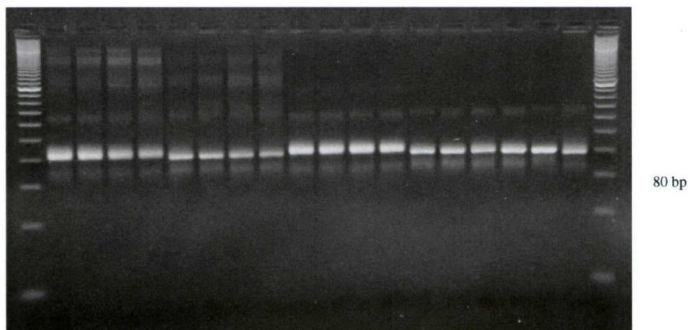
Figure 6 Separation of dsDNA from the DNA library into ssDNA by means of streptavidin magnetic beads, followed by PCR amplification of the ssDNA. Various amounts of beads of 100 \mu g (lane 2, 6, 10 and 14), 200 \mu g (lane 3, 7, 11 and 15), 400 \mu g (lane 4, 8, 12 and 16) and 600 \mu g (lane 5, 9, 13 and 17) were used. Amplification products of the ssDNA that was originally coupled to the magnetic beads (lanes 2-5) and those of the ssDNA that was originally not coupled to the magnetic beads (lanes 10-13) are present. The corresponding blanc assay to which no DNA was added are shown in the lanes 6-9 and lanes 14-17, respectively. Lanes 1 and 20 are the Super-ladder-Low 20bp Ladder (50 bands: 20bp-1000bp in exact 20bp increments, brighter bands at 200bp and 500bp). Products in the lanes 18 and 19 are not part of the experiments performed within the scope of this project.
