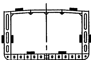
SECTION AT MIDSHIPS
