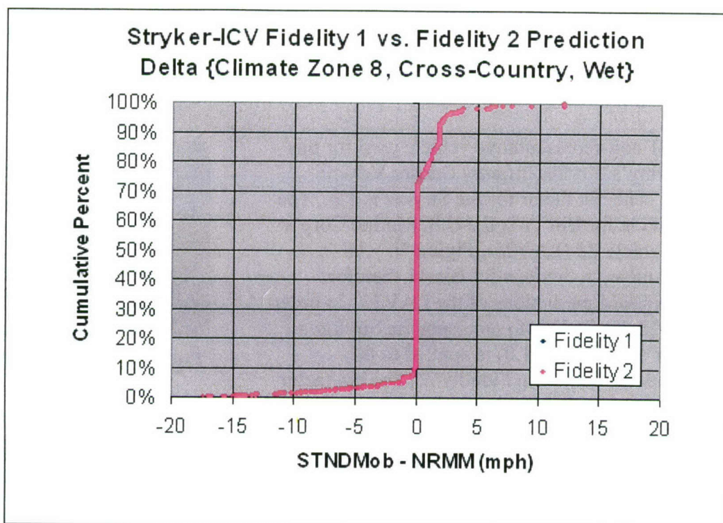
Figure 77. Stryker-ICV Fidelity 1 vs. Fidelity 2 Prediction Delta {Climate Zone 8, Cross-Country, Wet}.
