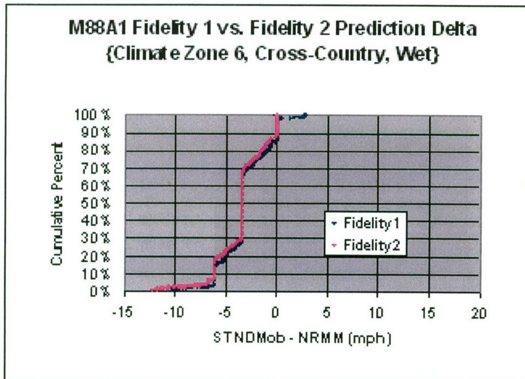
Figure 36. M88A1 Fidelity 1 vs. Fidelity 2 Prediction Delta {Climate Zone 6, Cross-Country, Wet}.
