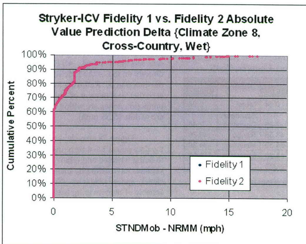
Figure 78. Stryker-ICV Fidelity 1 vs. Fidelity 2 Absolute Value Prediction Delta {Climate Zone 8, Cross-Country, Wet}.
