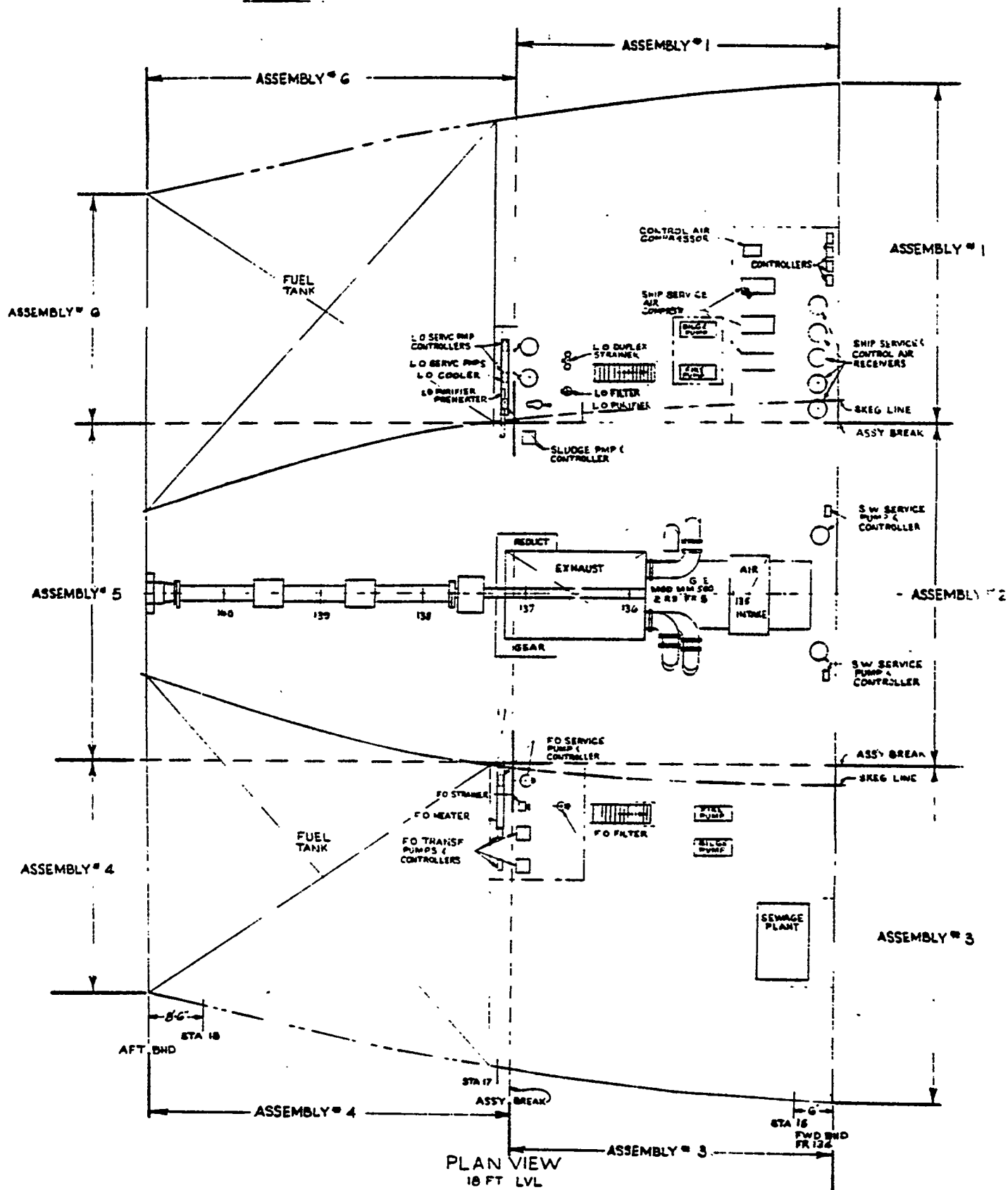
Figure 4-5. Heavy Duty Gas Turbine Arrangement (Sheet 2 of 5)
