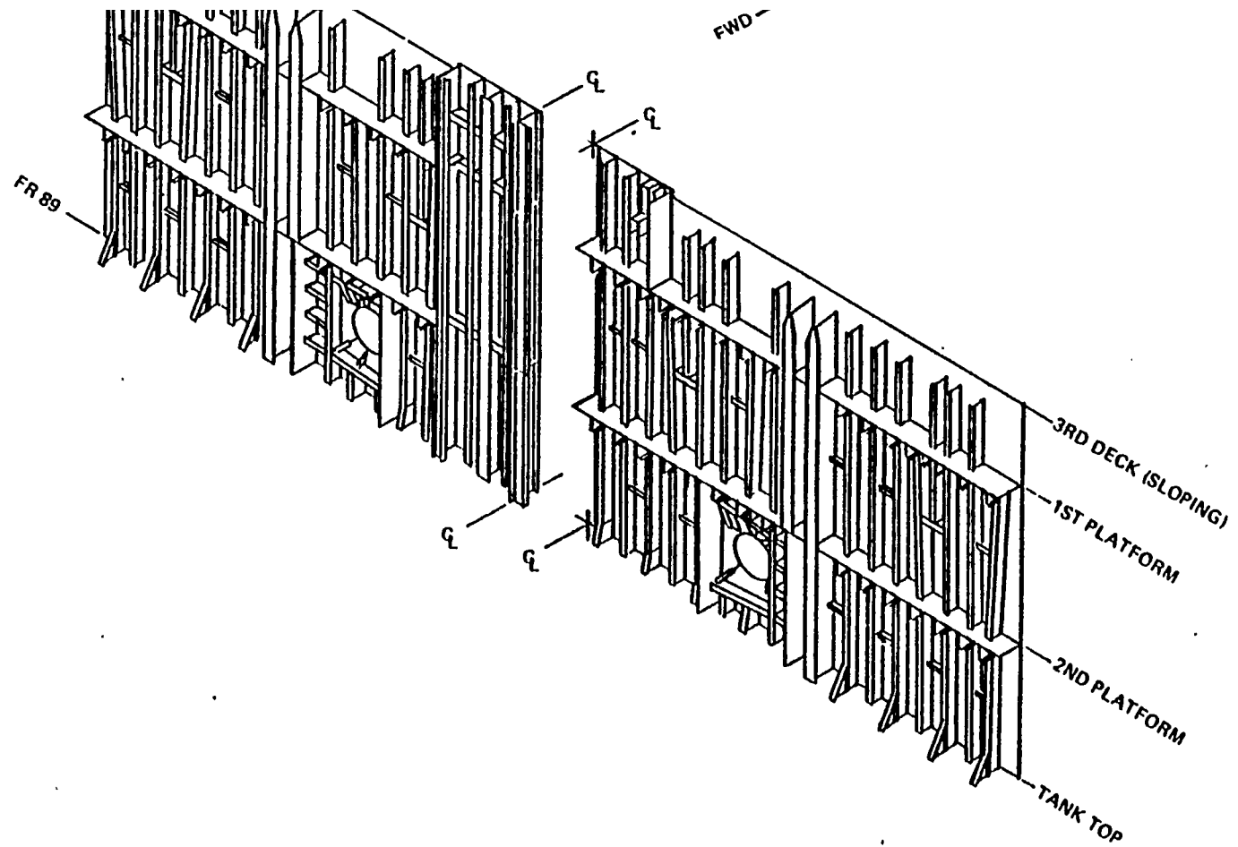
Figure 7-11. Three Dimensional Projection Showing Relationship of Subassemblies
