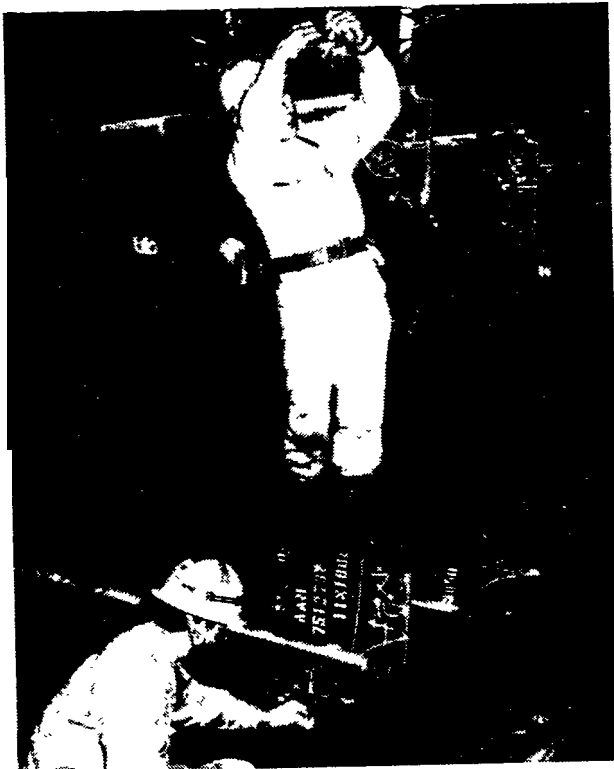
FIGURE 6-15: Specific A/C procedure apply to: A. Checking a measurement between panel and bracket edges in a sub-block. B. Checking a measurement between the edges of a panel and internal structure in a block. C. Checking alignment of a tank-top panel relative to a bottom-shell panel in a block. D. Monitoring bottom alignment between keel laying and launching. The distance measured is that from the bottom shell to a reference line marked on the vertical angle-iron which is fixed to the dock floor.
