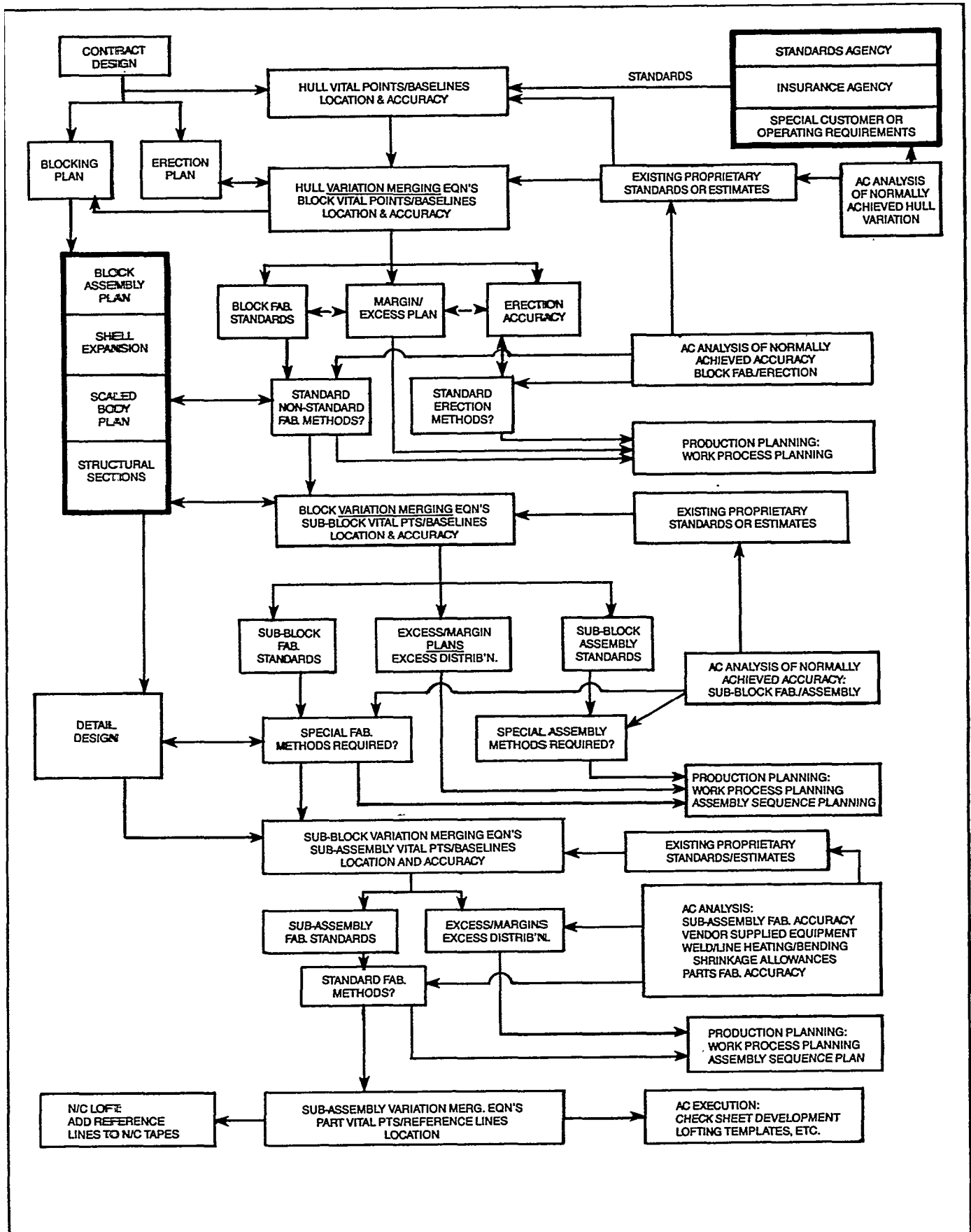
FIGURE 3-1: An A/C Planning Process.
