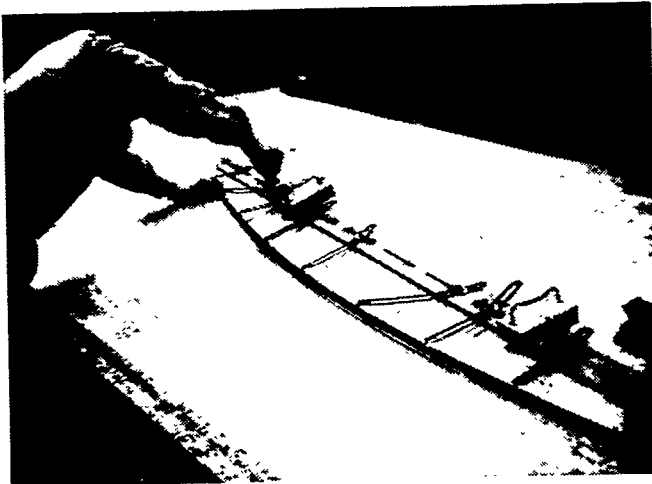
FIGURE 6-7: A. Semi-automatic (shown) and manual line heating methods are applied as controlled work processes for forming curved plates. Similar techniques are also used after rolling or bending to refine the curvature achieved. Line heating is not limited by furnace size, as for forming by a blacksmith, nor limited by press and roller capacities. Thus, line heating is being applied to increasingly wider and longer plates as a means for reducing the lineal footage of welding required and associated shrinkage which complicates A/C. B. Loftsmen prepare for each part, a family of sight-line templates on a single Mylar sheet and thereafter, as one option, reproduce the templates in wood. Each template features a vertical member having one side designated as a sight face and on which appears a sight-line mark, "<". Match marks are provided on the bottom of each template to coincide with plate edges. A station number and angle of inclination relative to the plate surface, when curved, are noted on each template. C. Some part-fabrication shops directly employ a "Mylar" for setting a family of adjustable sight-line templates. D. Transverse curvature is checked by measuring the distances between each template's curved edge and the plate surface between applications of line heating. Correct twist is obtained when the sight faces of all templates are in the same plane. Proper longitudinal curvature is achieved when the sight-line marks all coincide with a taut string.
