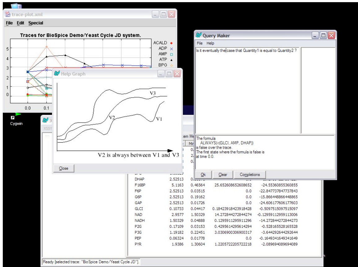
Figure 2. A screenshot of the Simpathica/XSSYS Natural Language Interface. The “Query Maker” window is used to type in English queries. A Help System showing the intuitive meaning of typical queries can be also consulted to facilitate the expression of the Temporal Logic queries.
