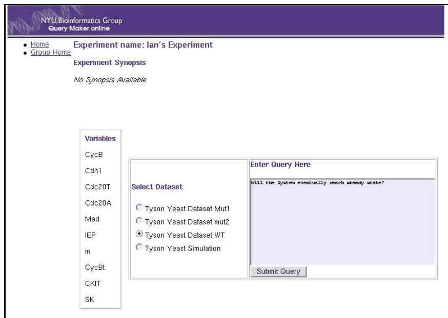
Figure 4. Once an experiment has been selected, QMO shows a page with a list of the “variables” appearing in each of the datasets from the experiment. The user can enter a query involving those variables in the text area on the right.
