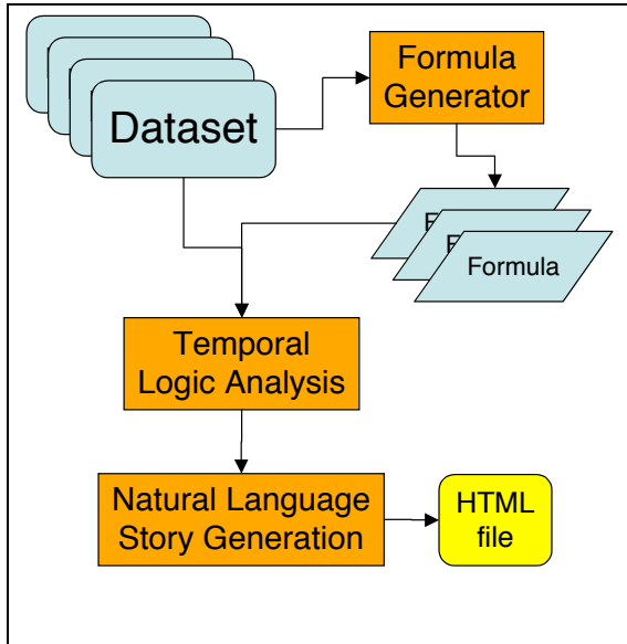
Figure 6. The architecture of the “biologically interesting factoid” generation system. Given a number of datasets (logically belonging to a given “experiment”, the system generates a set of CTL formulae using a number of carefully chosen heuristics (to constrain the number of formulae being generated). Each formula is fed to the temporal logic analyzer XSSYS, which is essentially a restricted model-checker, and the results of such analysis is then fed to the Natural Language Generation system which finally produces an HTML formatted file.
