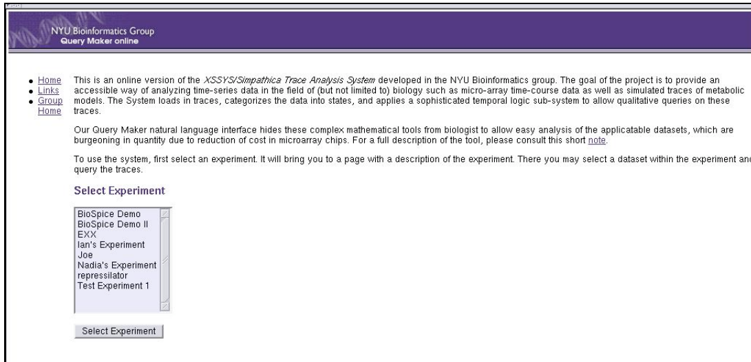
Figure 3. This is the opening page of the “Query Maker Online” (QMO) system viewable at http://bioinformatics.nyu.edu:3001/Projects/qmo/lasp/home . The system shows a list of the “experiments” for which the NYUSIM database has datasets visible to the general public.
