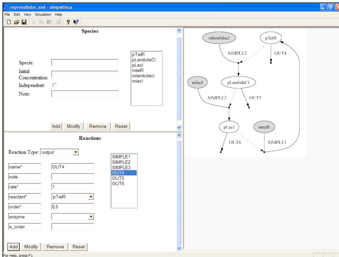
Figure 1. The Simpathica Main Window. The system being analyzed is the “repressilator” circuit (EL00). The top left frame contains a list of the reactants. The bottom left frame is used to insert different kinds of reactions selected from a list of known reactions. Finally the right frame contains a depiction of the reactions' network.
