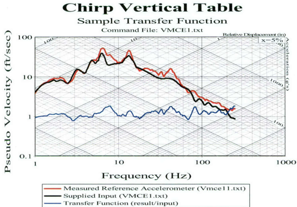
Figure 9. Comparison of Chirp Test Inputs and Requested Inputs
