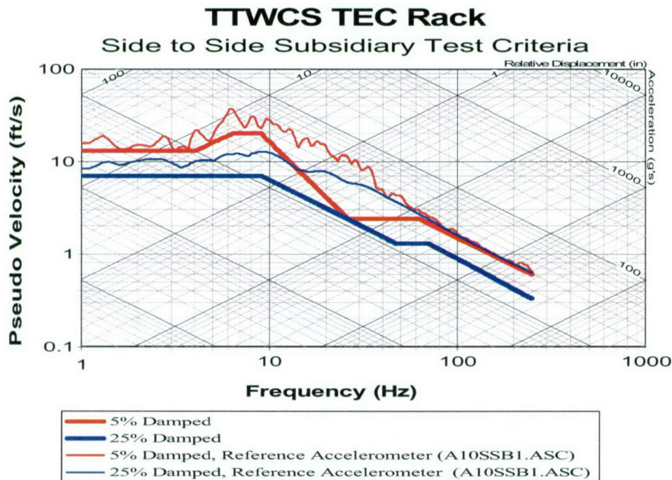
Figure 4. Side-Side Data Derived from TTWCS TEC Testing
