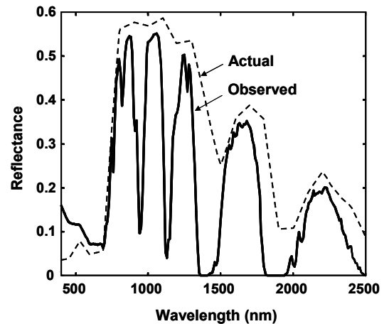
Figure 1. MODTRAN calculation of the apparent reflectance of a vegetation pixel as observed from space with nadir viewing, a Mid-Latitude Summer model atmosphere, and a Rural aerosol with visibility=23km.
