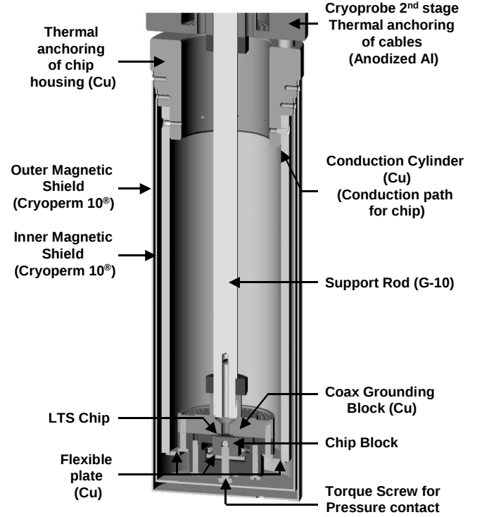
Fig. 5. The construction details of the chip housing.
