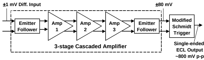
Fig. 9. A SiGe HBT amplifier chain, consisting of a three-stage cascaded differential amplifier with emitter follower buffers and a modified Schmidt trigger, designed to convert the mV-level differential digital output from LTS chips to V-level single-ended ECL signal.
