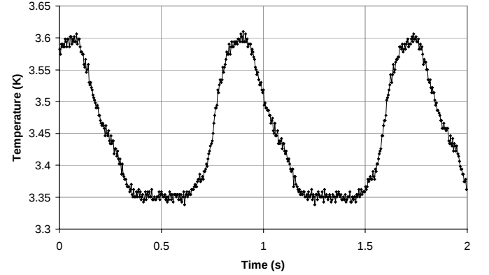
Fig. 3. Measured temperature oscillation of the Sumitomo cryocooler operating with a dc voltage standard chip.
