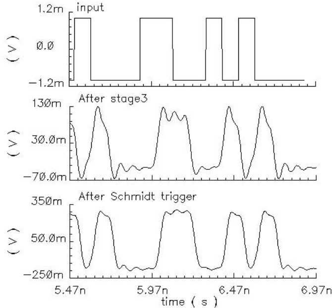
Fig. 16 Simulated time-domain response of the amplifier chain to 10 Gbps NRZ data pattern, showing the input (top), the output after the third stage of linear amplification (middle), and the final output after the Schmidt trigger (bottom).
