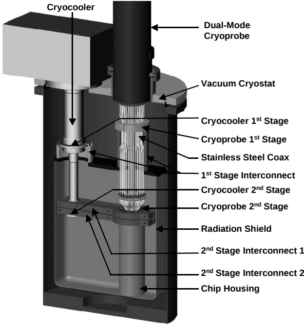
Fig. 4. Cut-away view of the complete cryopackage assembly.
