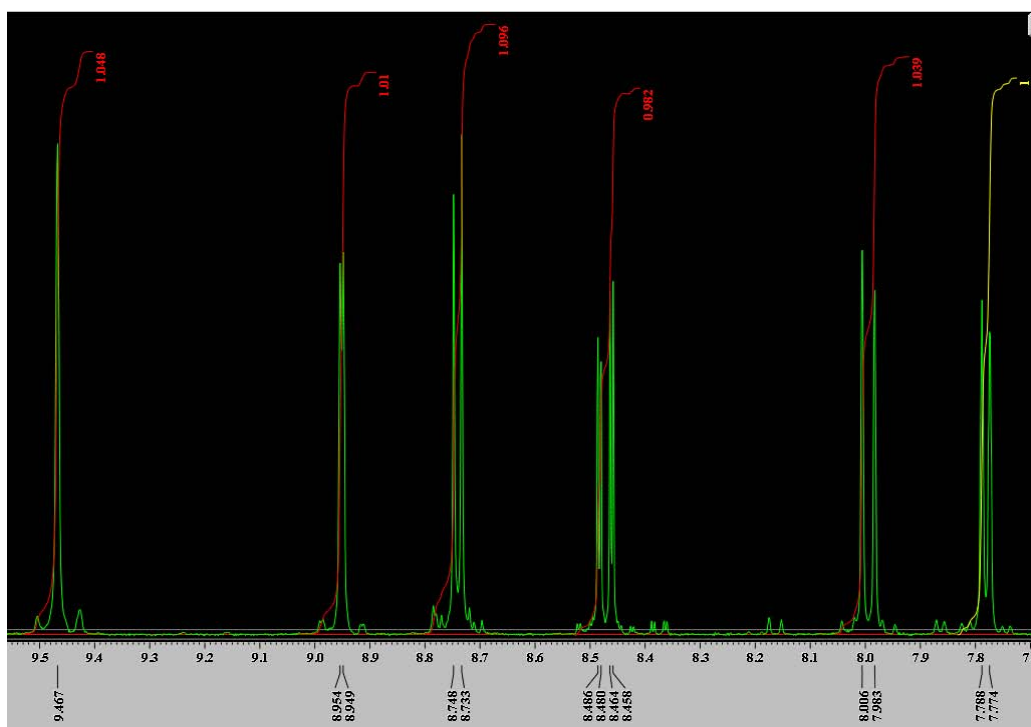
Figure 19 – ^1\text{H} NMR Spectra of Compound 3.
