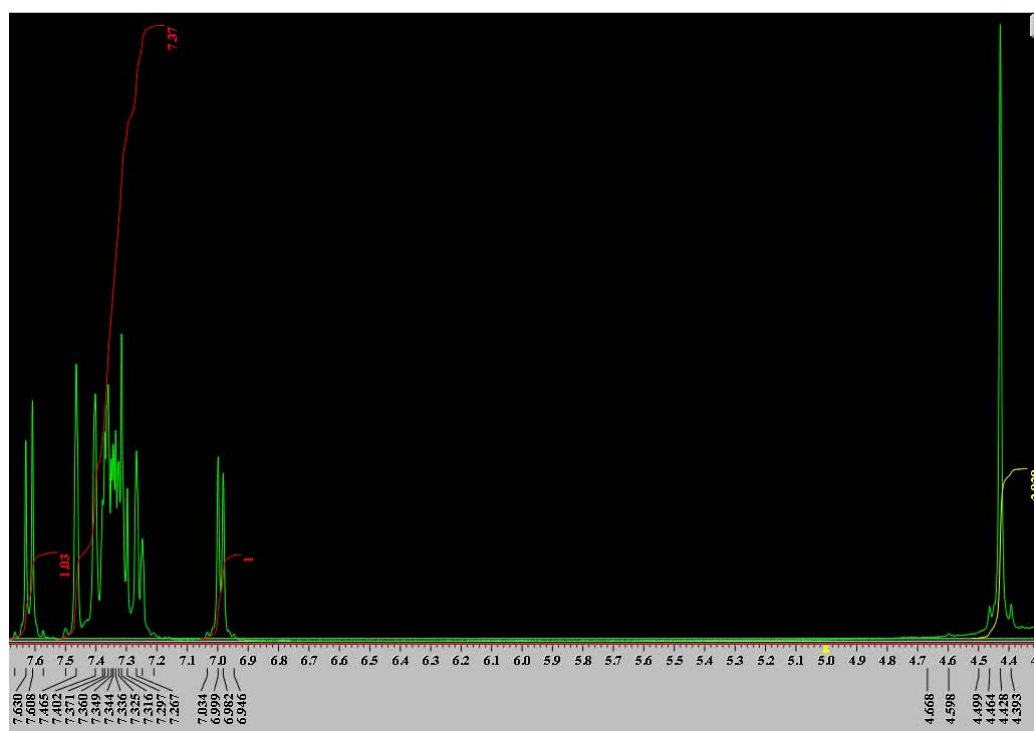
Figure 33 – ^1\text{H} NMR Spectra of Target 3 HCl Salt.
