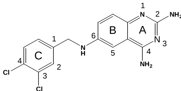
Figure 5 – 2,4-Diamino-6-[(3,4-dichlorobenzyl)amino]quinazoline.
