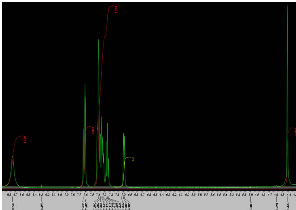
Figure 32 – ^1\text{H} NMR Spectra of Target 2 HCl Salt.
