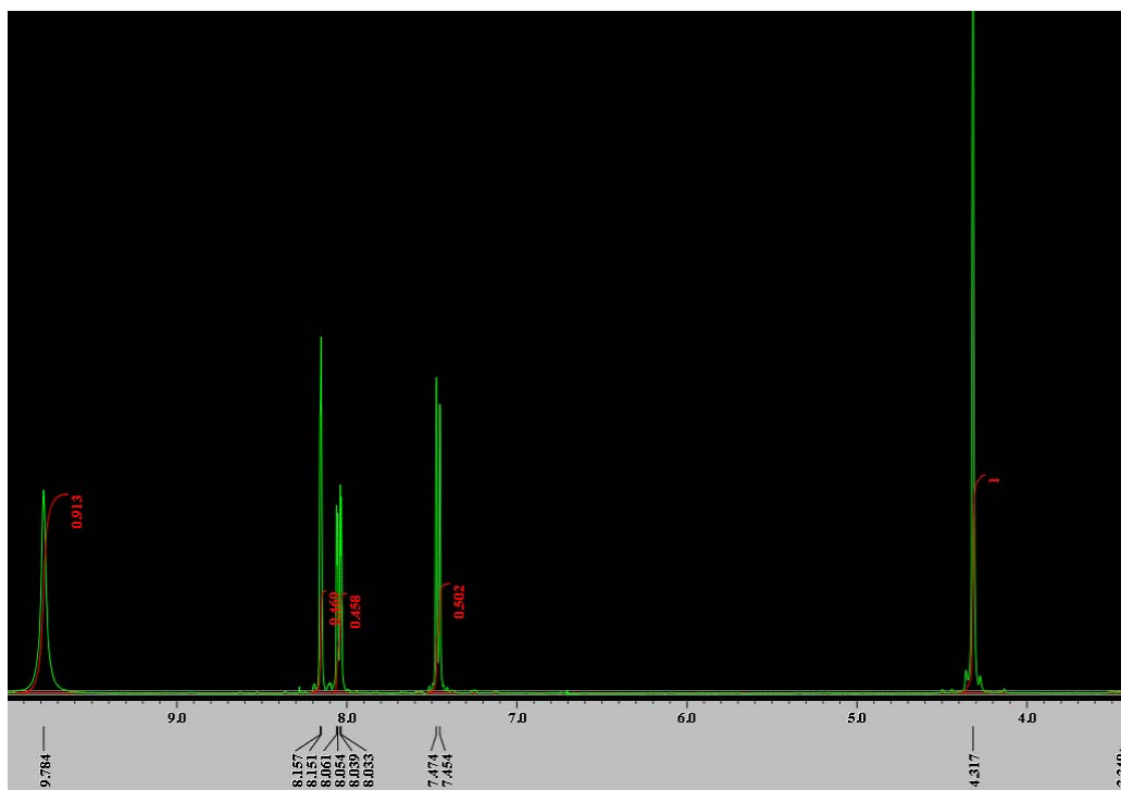
Figure 18 – ^1\text{H} NMR Spectra of Compound 2.
