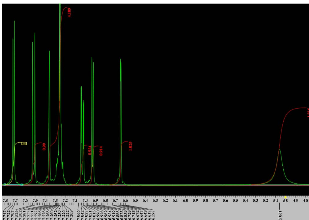
Figure 27 – ^1\text{H} NMR Spectra of Target 3.
