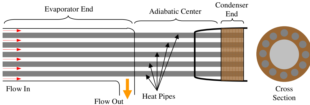
Figure 3-6. Conceptual sketch of the transfer loop-Stirling heat pipe interface (not to scale).
