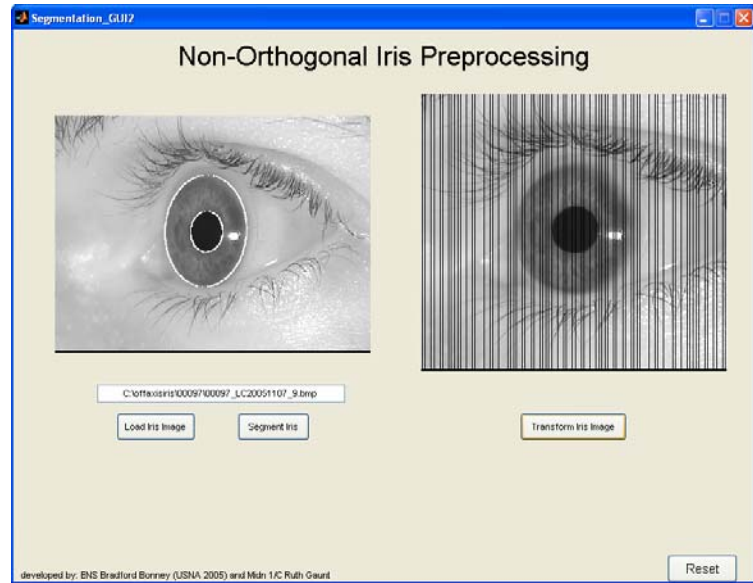
Figure 12. Preprocessing GUI.
