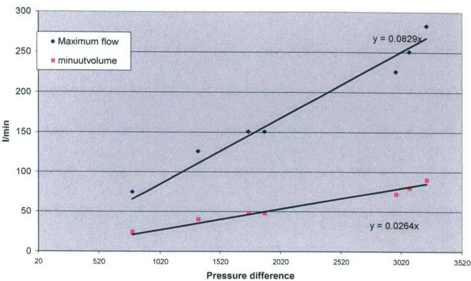
Figure A.1 Calibration lines for maximum and minute volume as measured for the old system. Data was generated on a dummy head using a breathing machine.
