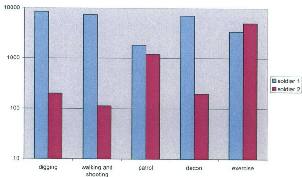
Figure 12 Average protection values of the Porton Down field trial 2003. Soldier 1 is Aage; Soldier 2 is Gerard, both wore the old and the new system alternating.
