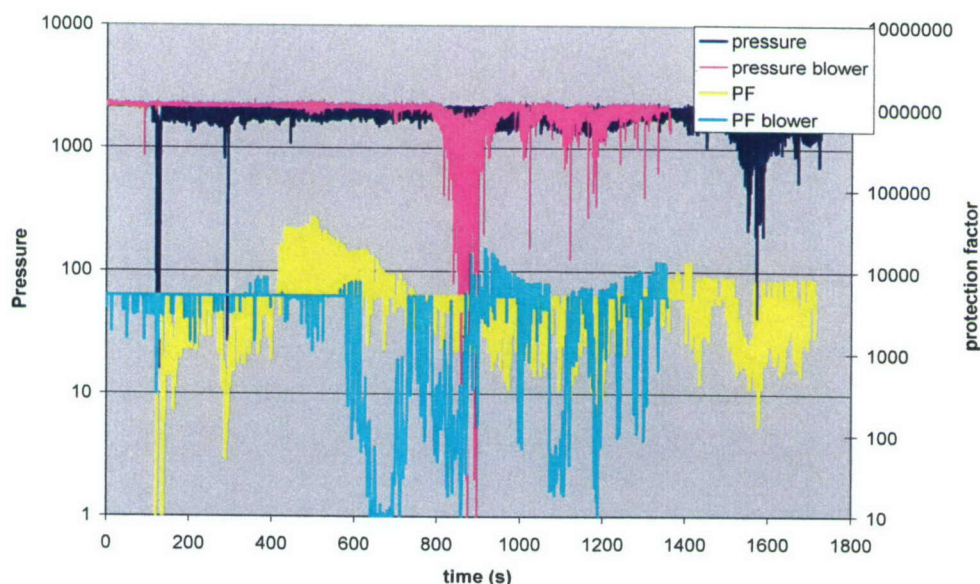
Figure 13 Results of the standard-protocol both with and without blower.
