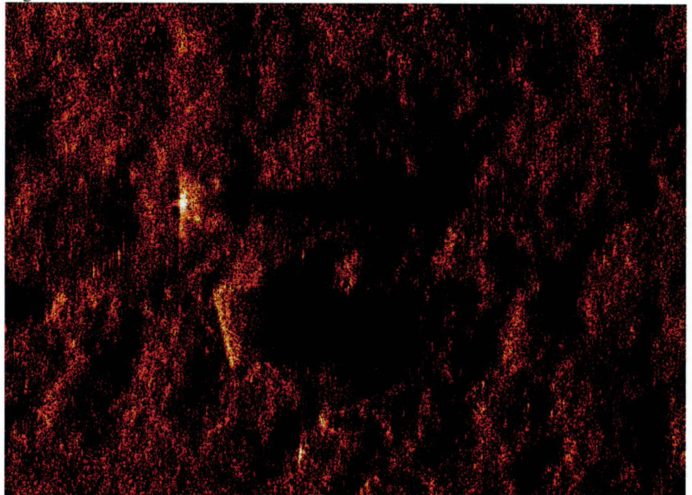
Figure 5.1: SAS image of a sphere (upper target) and a cylinder (lower target) at 75 m range from a 10 m long rail.
