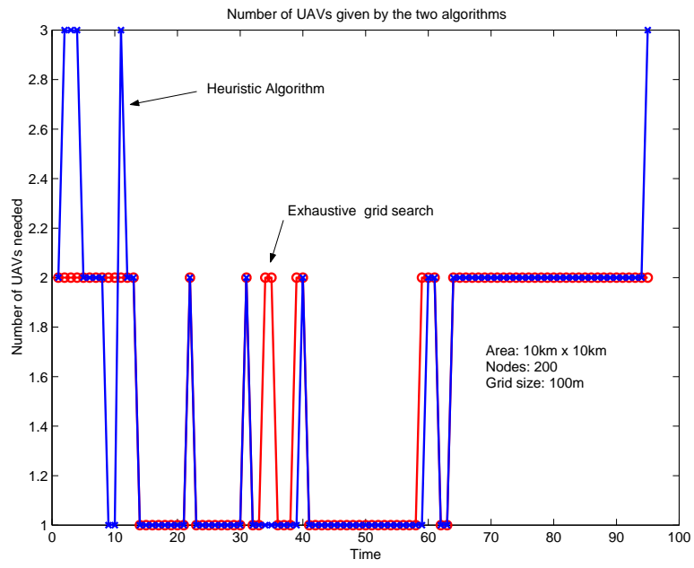
Fig. 5. Comparison of the number of UAVs given by the Grid and our heuristic algorithm
