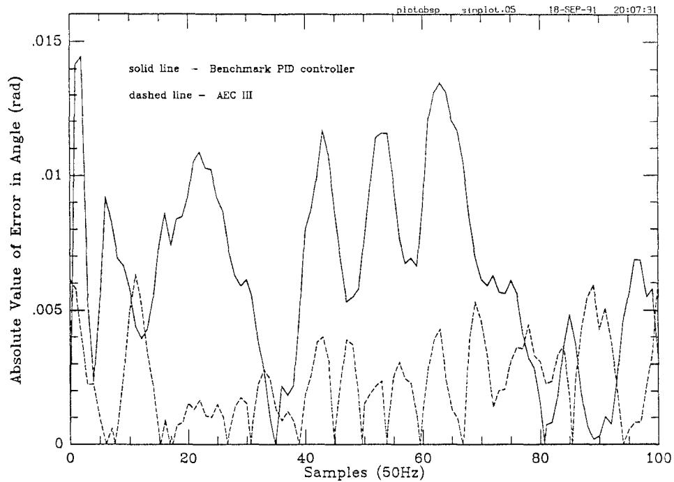
Figure 9: Position Error for AEC III Compared to Benchmark PID Controller they went out of a predefined range as suggested by [Craig, 1988].
