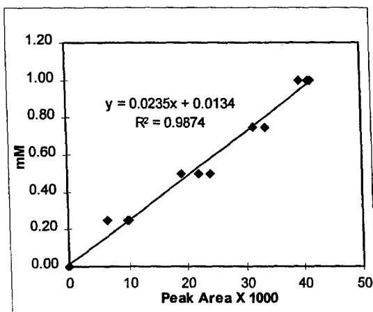
Figure 6. M-22 Concentration Standard Curves
