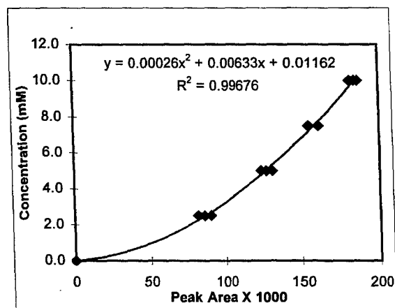
Figure 6. M-22 Concentration Standard Curves
