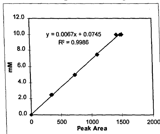
Figure 2. M-1 Concentration Standard Curves
