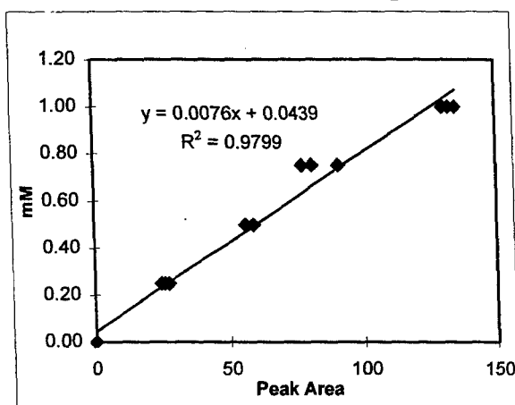
Figure 2. M-1 Concentration Standard Curves
