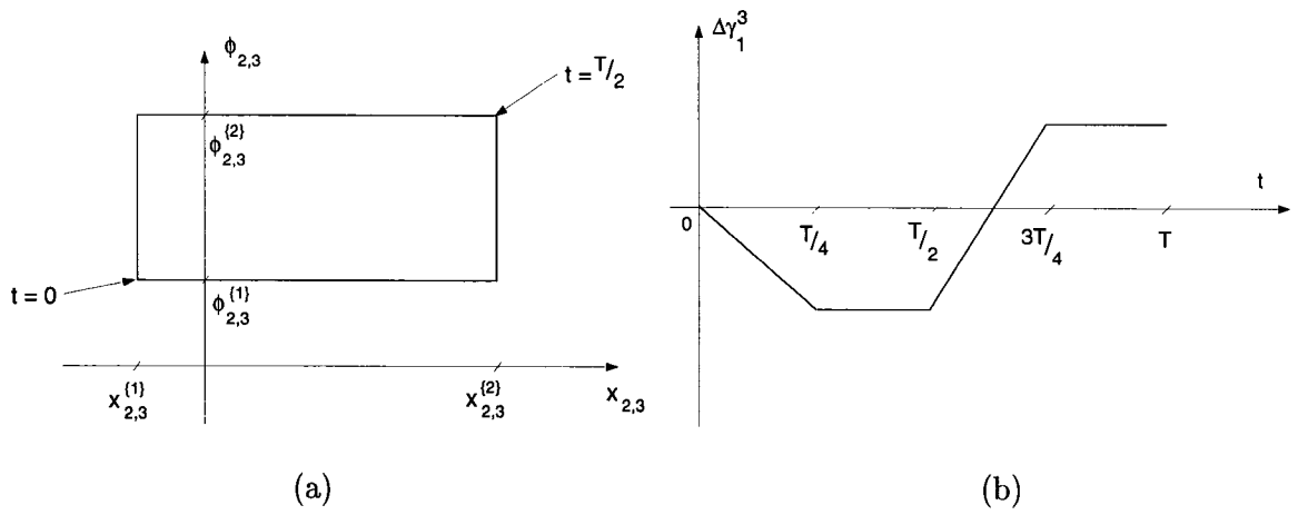
Fig. 5.3.6: Piecewise Constant Controls and Geometric Phase for Translating 2-module NVGT
