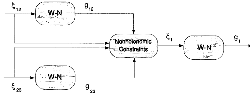
Fig. 5.3.5: The 2-module NVGT Model for Motion Control
