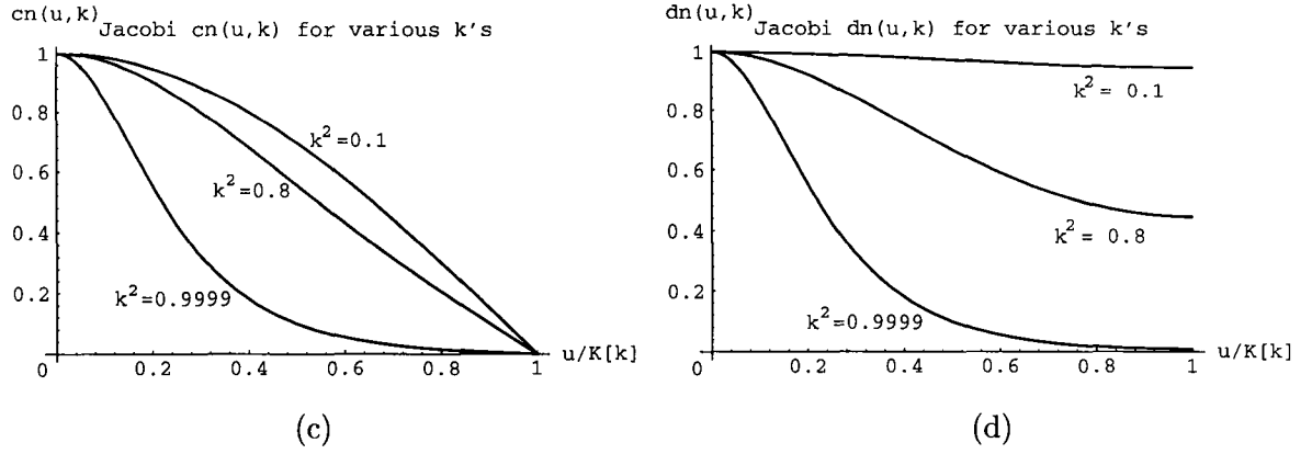
Fig. 2.2.1: Jacobi Elliptic Functions
