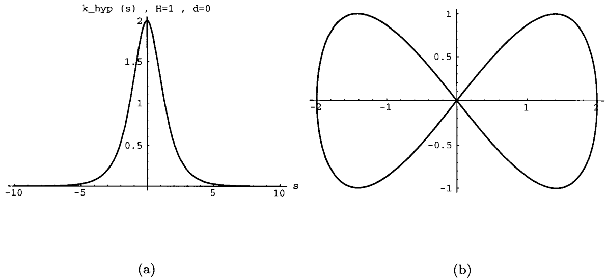
Fig. 3.2.5: Solutions of the Bryant-Griffiths Optimality Constraint when H = C
