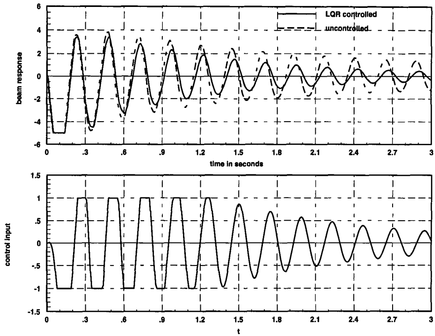
Figure 6.8: Response of the beam under LQR control
