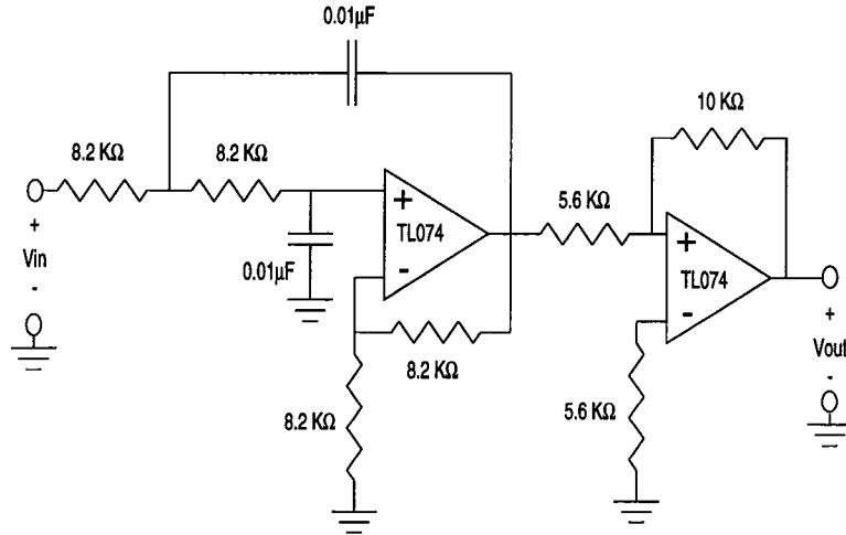
Figure 6.3: Low pass filter schematic
