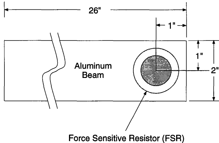
Figure 8.1: Mounting of the FSR (force sensitive resistor)
