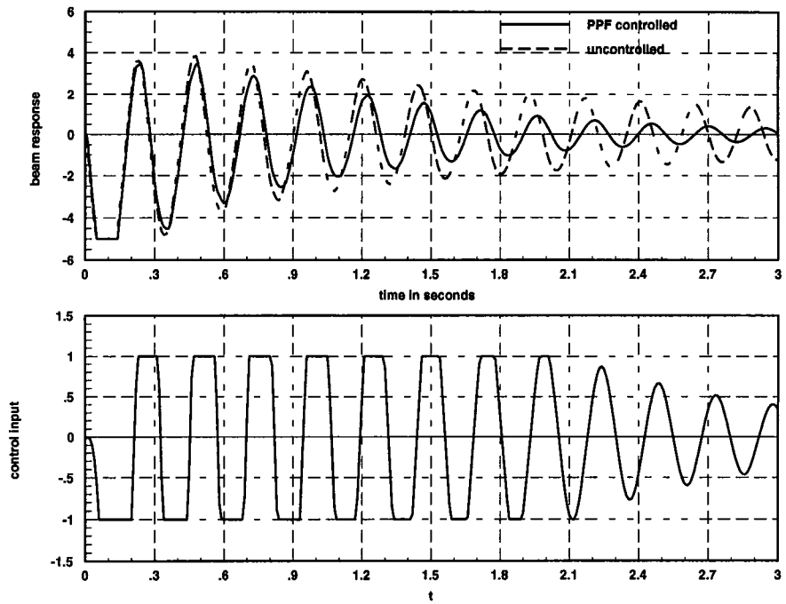
Figure 6.10: Response of the beam under PPF control
