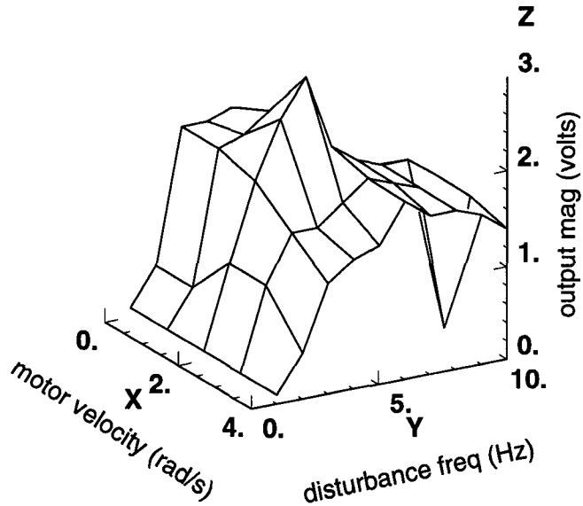
Figure 7.10: Disturbance response of beam using gain scheduling controller controllers depending on the motor velocity. That is use H_0(s) when \omega_m \leq 2 and use H_4(s) when \omega_m > 2 . This approach is a simple form of gain scheduling. The performance of this gain scheduling controller is depicted in Figure 7.10.
