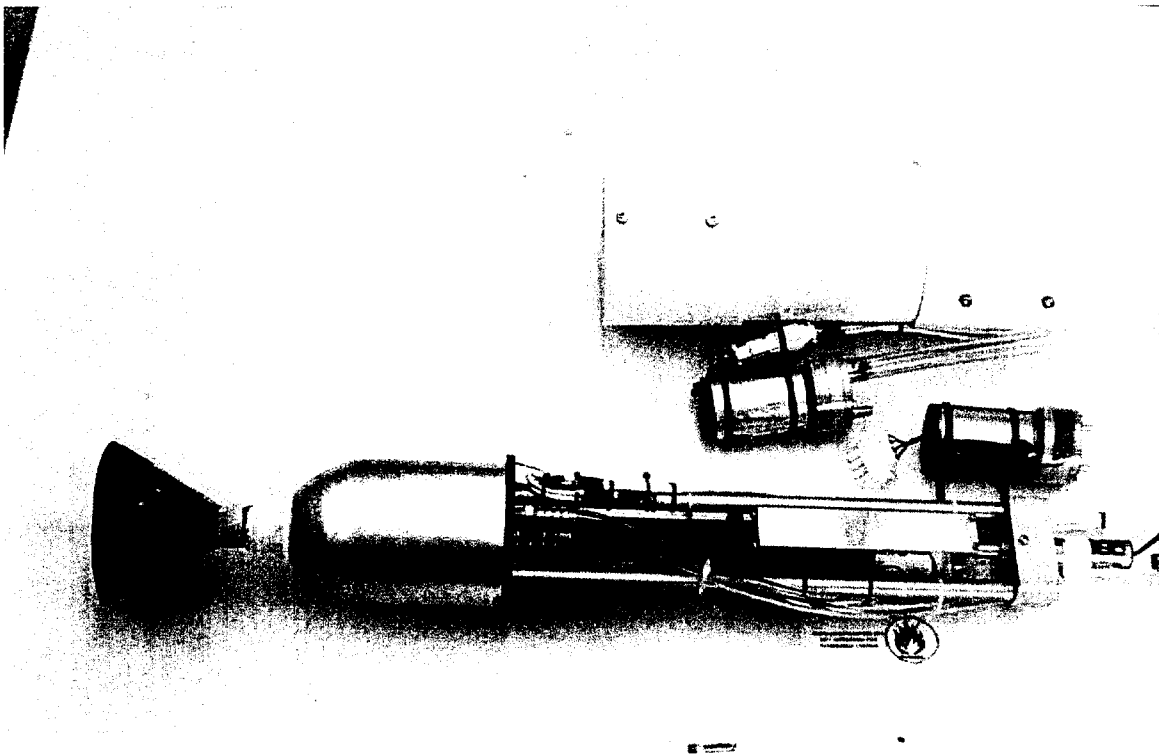
Figure 6. Detail of pump system (top) and cloudscope with faring removed (below)
