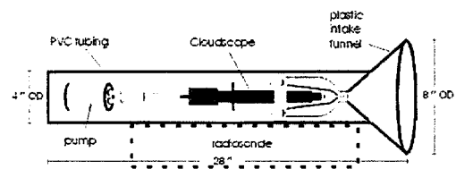
Figure 5. Schematic of cloudscope showing air sample intake faring.
