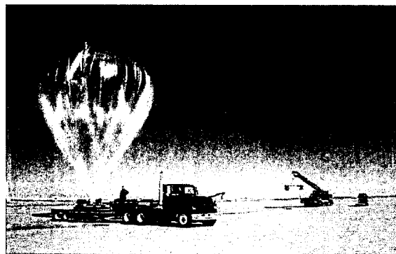
Figure 3. Launch test inflation.
