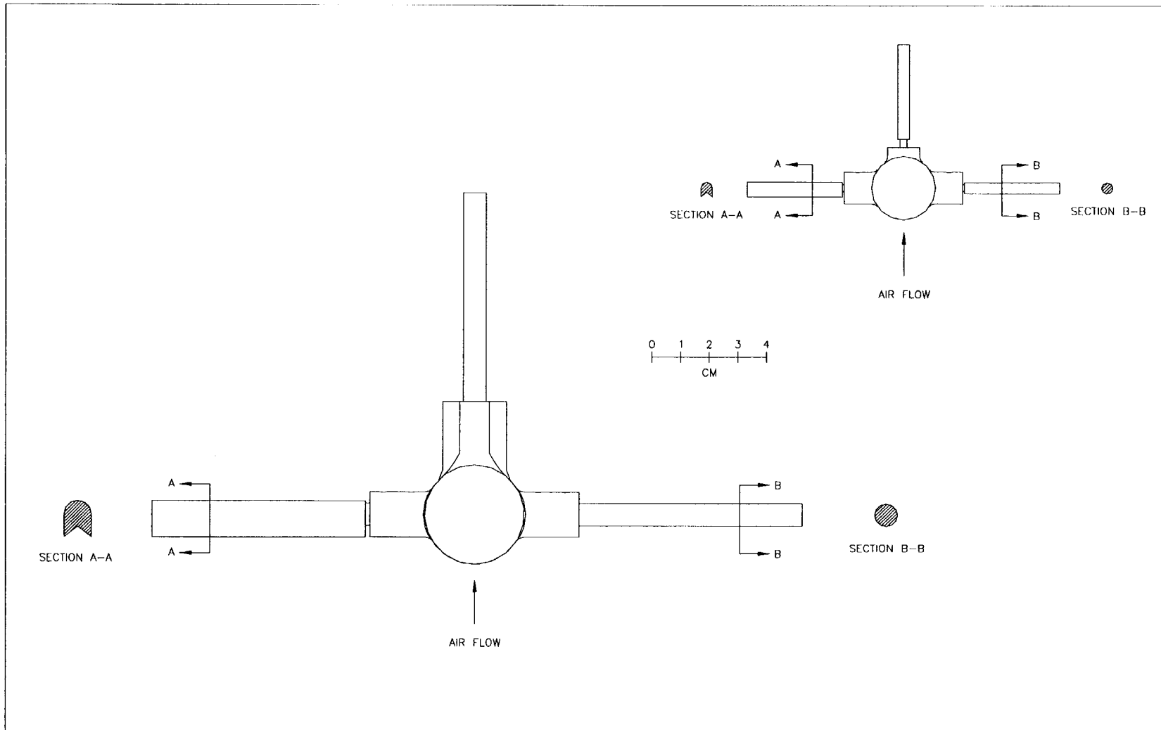
T probe showing air flow and sensor shapes for two similar shaped probes, large T, small T, having different impaction efficiency for different size. Each assembly has individual sensors with identical impaction efficiency for same size, shape and density particles.
