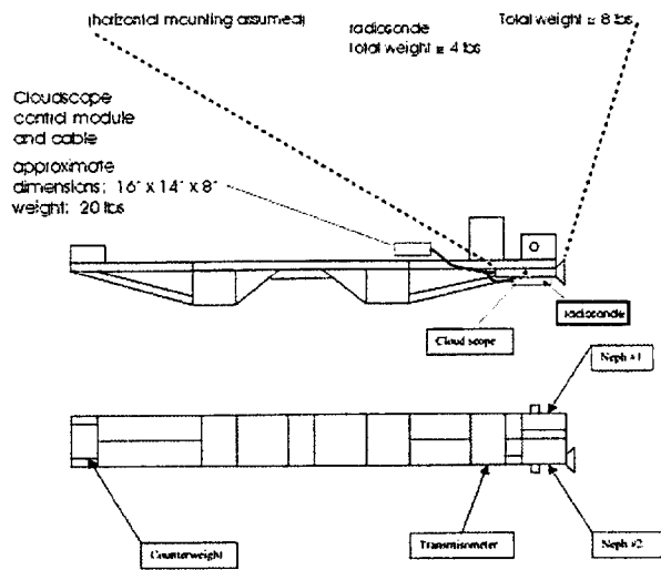
Figure 4. Layout of gondola instrumentation.
