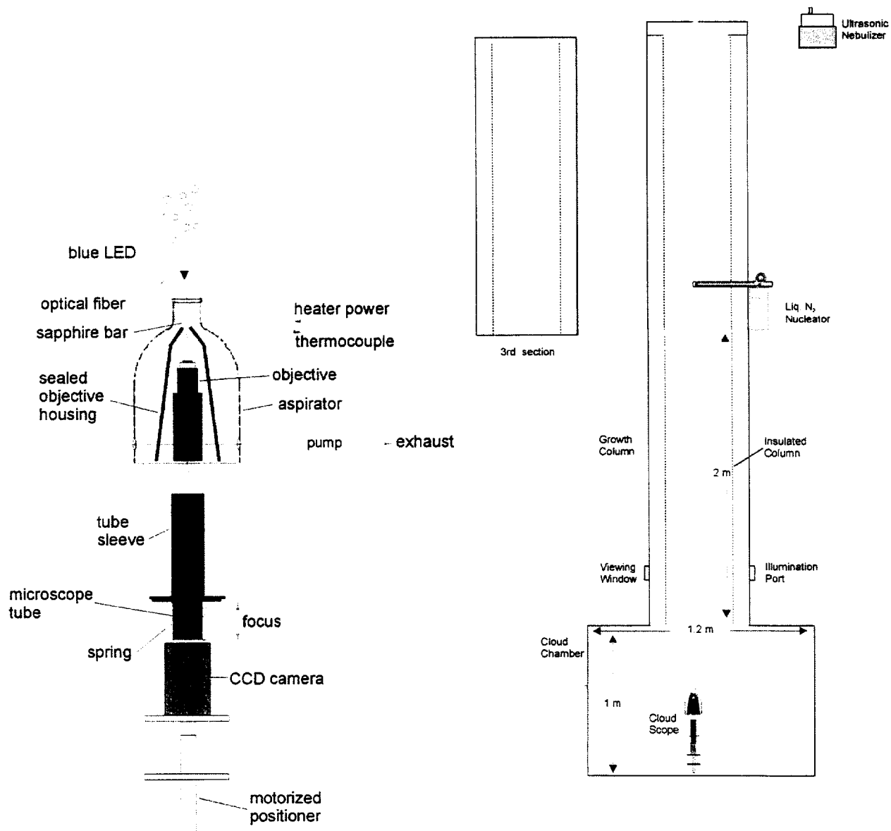
Schematic diagram of the experimental chamber.
