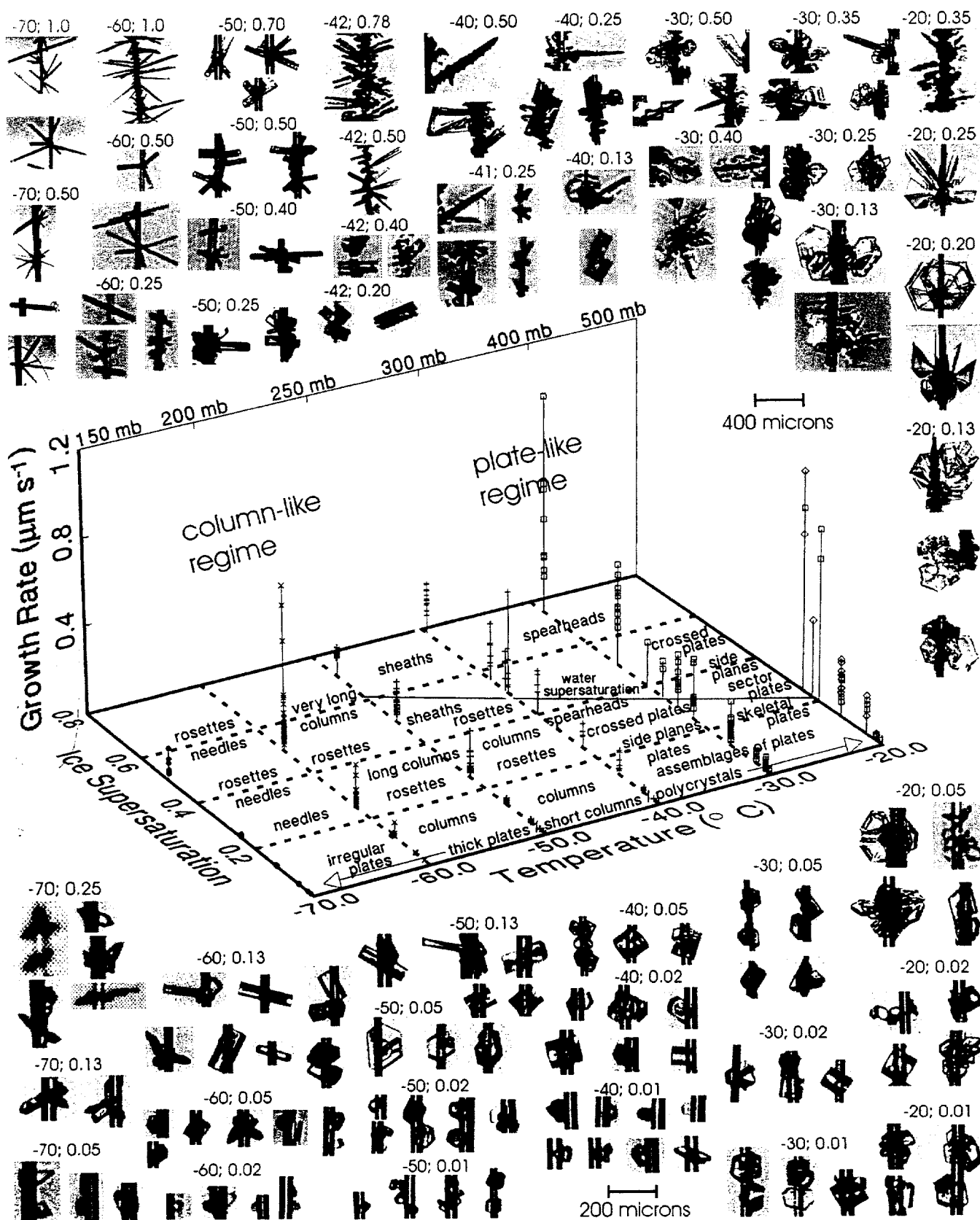
Figure 1. Map of ice crystal habit of crystals grown under cirrus conditions from -20C to -70C over a range of supersaturation typical of cirrus growth.
