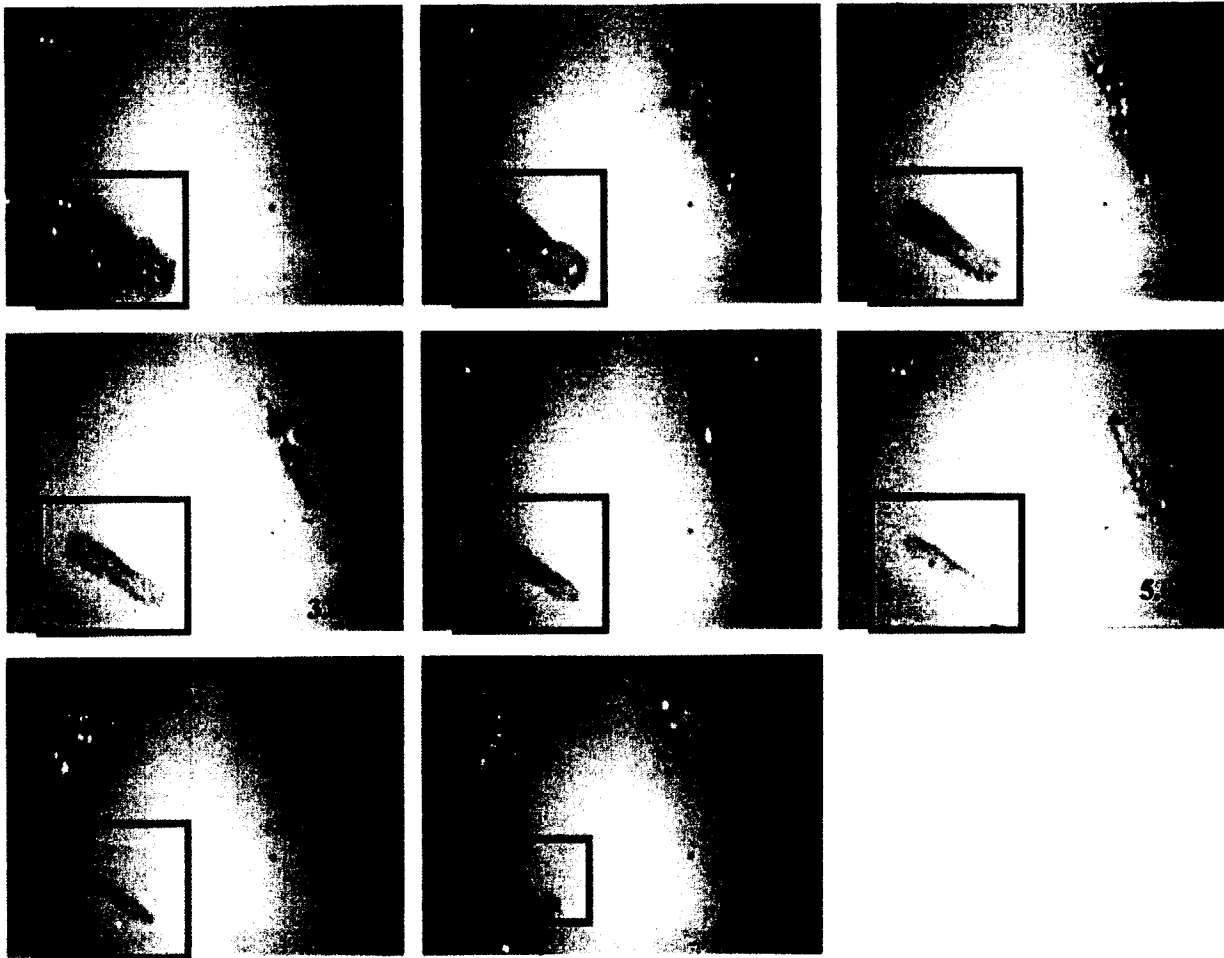
A rimed column. As it sublimated the rime is removed revealing the column.
