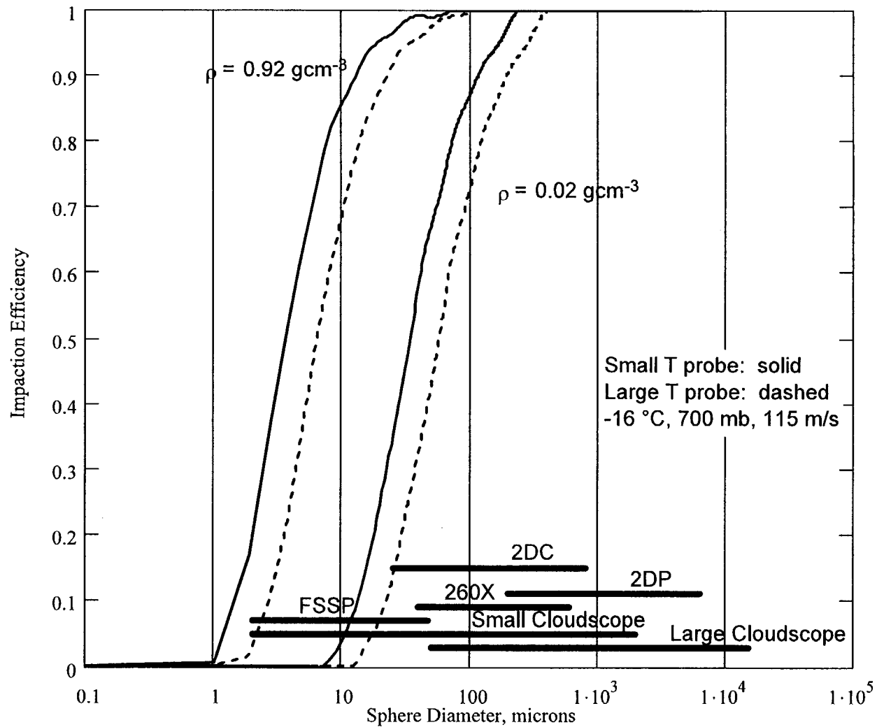
Impactation efficiency of spherical particles of different density for large and small T probes. Ranges of instruments for ancillary measurements are shown.
