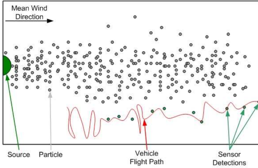
Figure 3.9: Maneuver decision based on single pheromone detection. Deciding to maneuver an aircraft based on a single detection is not the best odor-based navigation method, as it can easily keep the vehicle from entering the plume.
