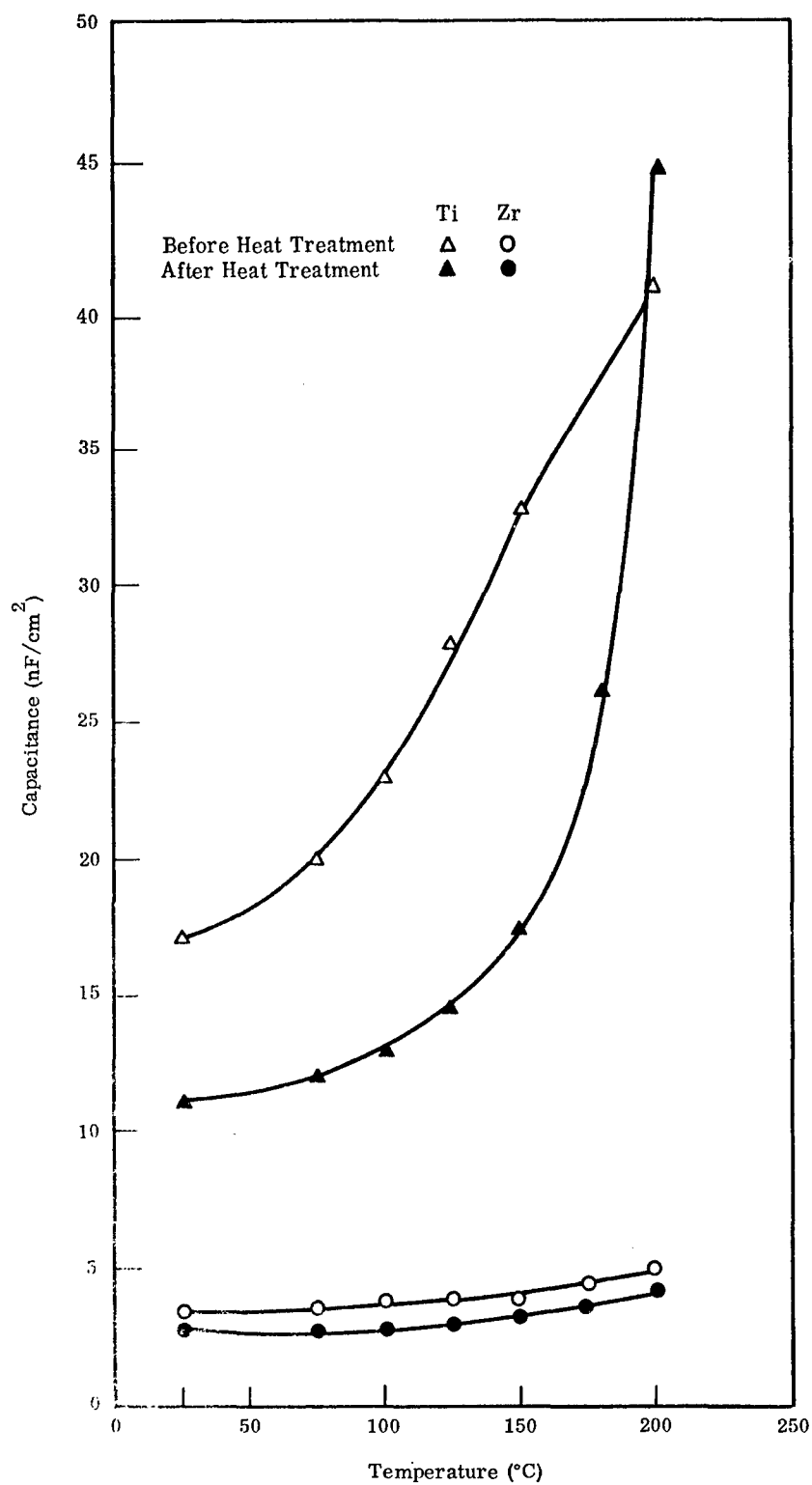
Fig. 2 Temperature-Capacitance Curve for Air Heated Films
