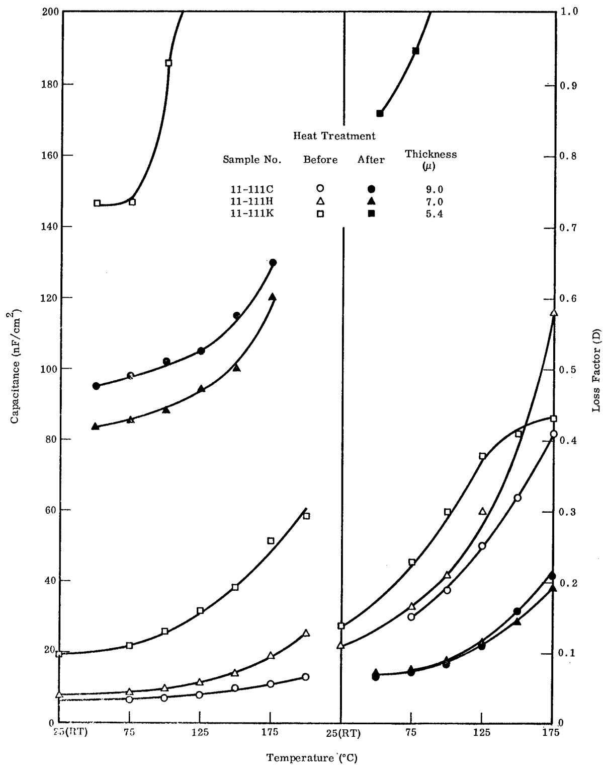
Fig. 3 Capacitance-Temperature Characteristics for Ti-Based Films
